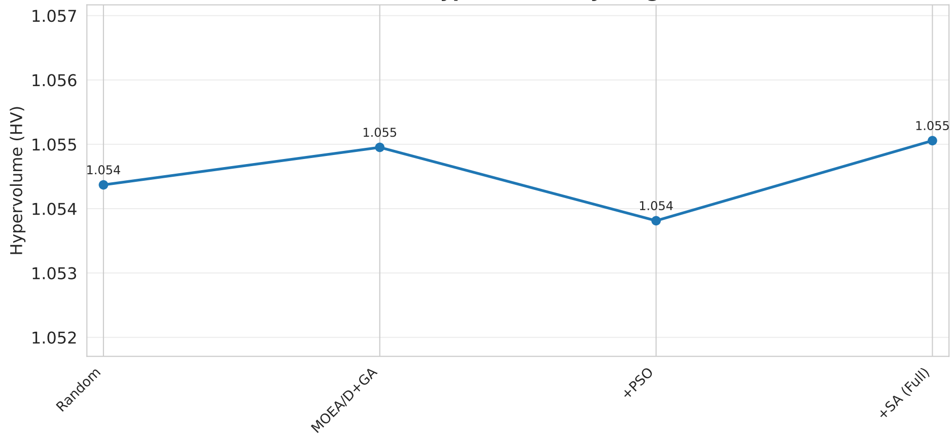
Final Hypervolume by Stage
