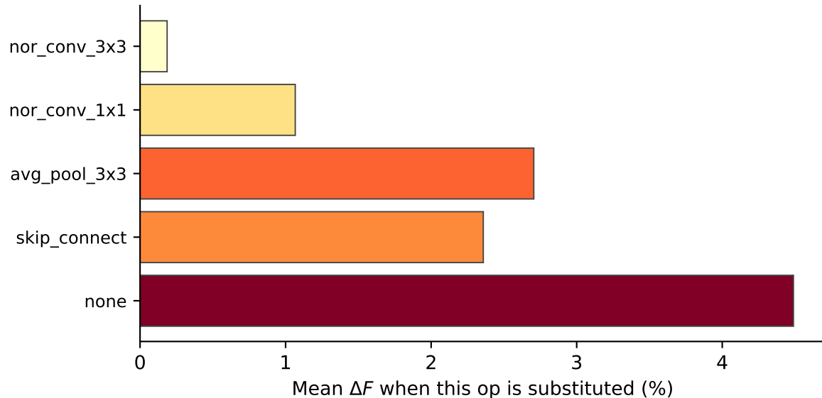
Per-Operation Disruption (How damaging is each replacement?)
