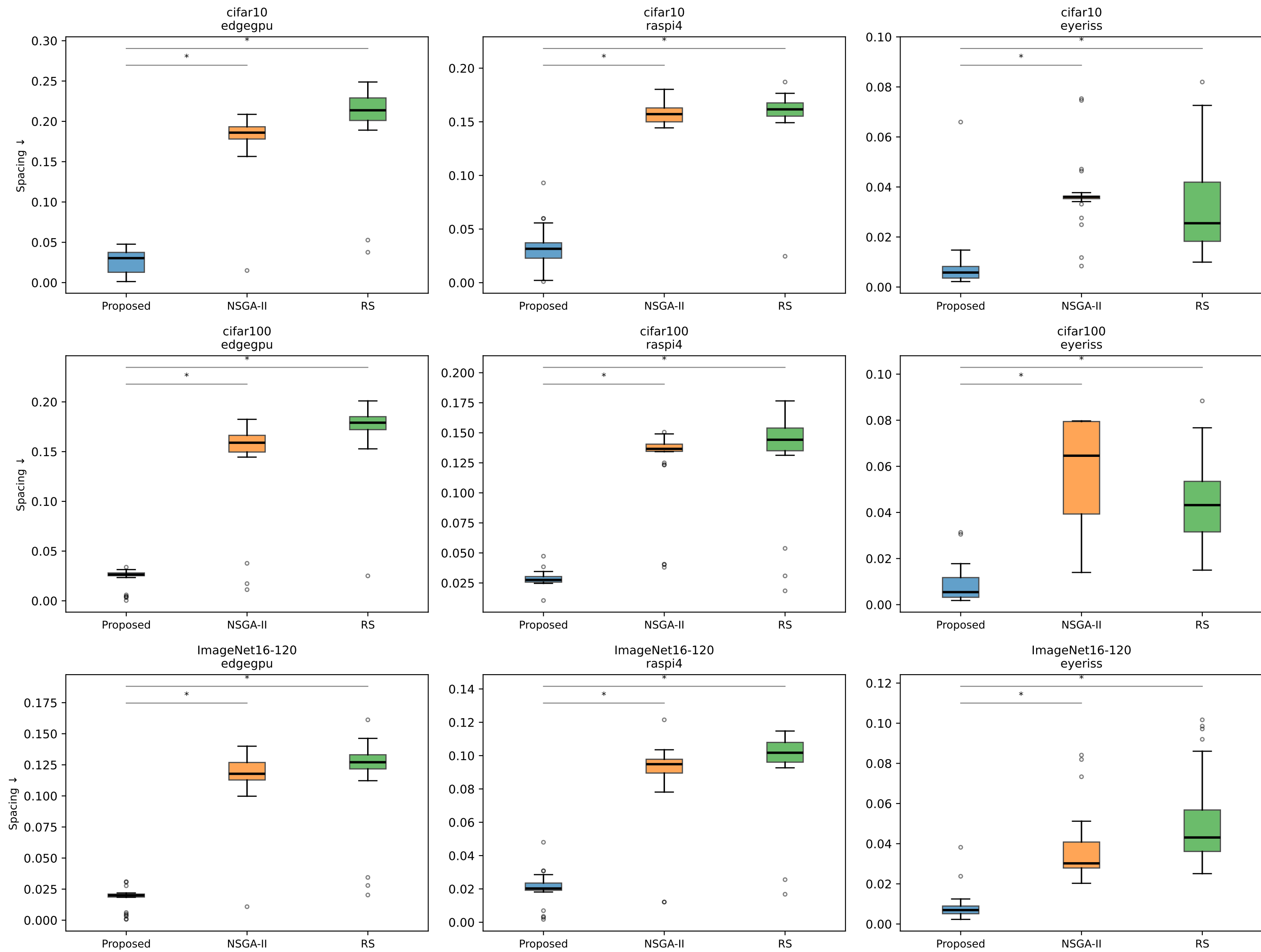
Spacing ↓ Distribution Across 30 Seeds (normalised [0, 1]^2 objective space)
