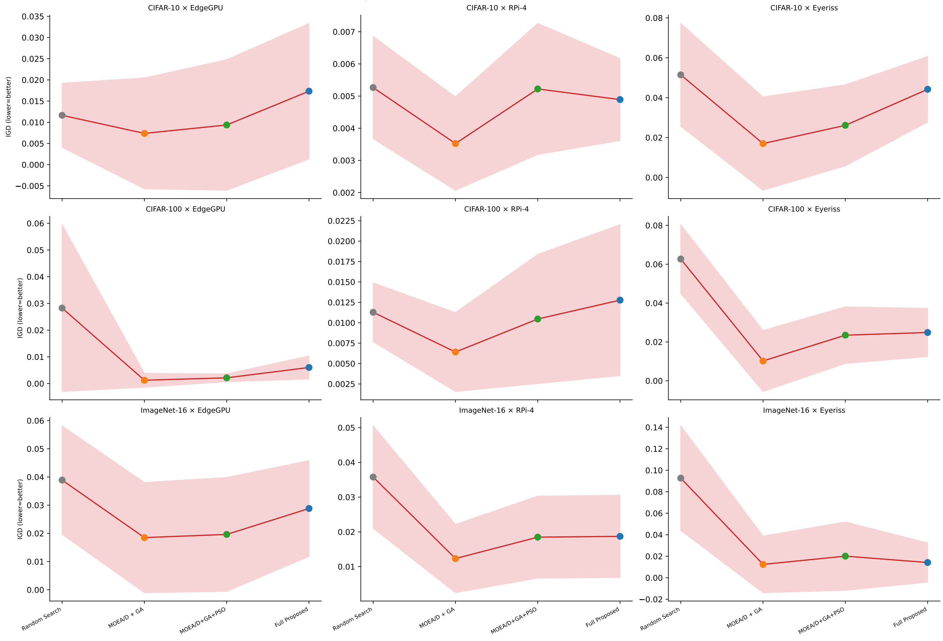
IGD Progression (Waterfall, mean \pm std, 30 seeds) — 3 \times 3
