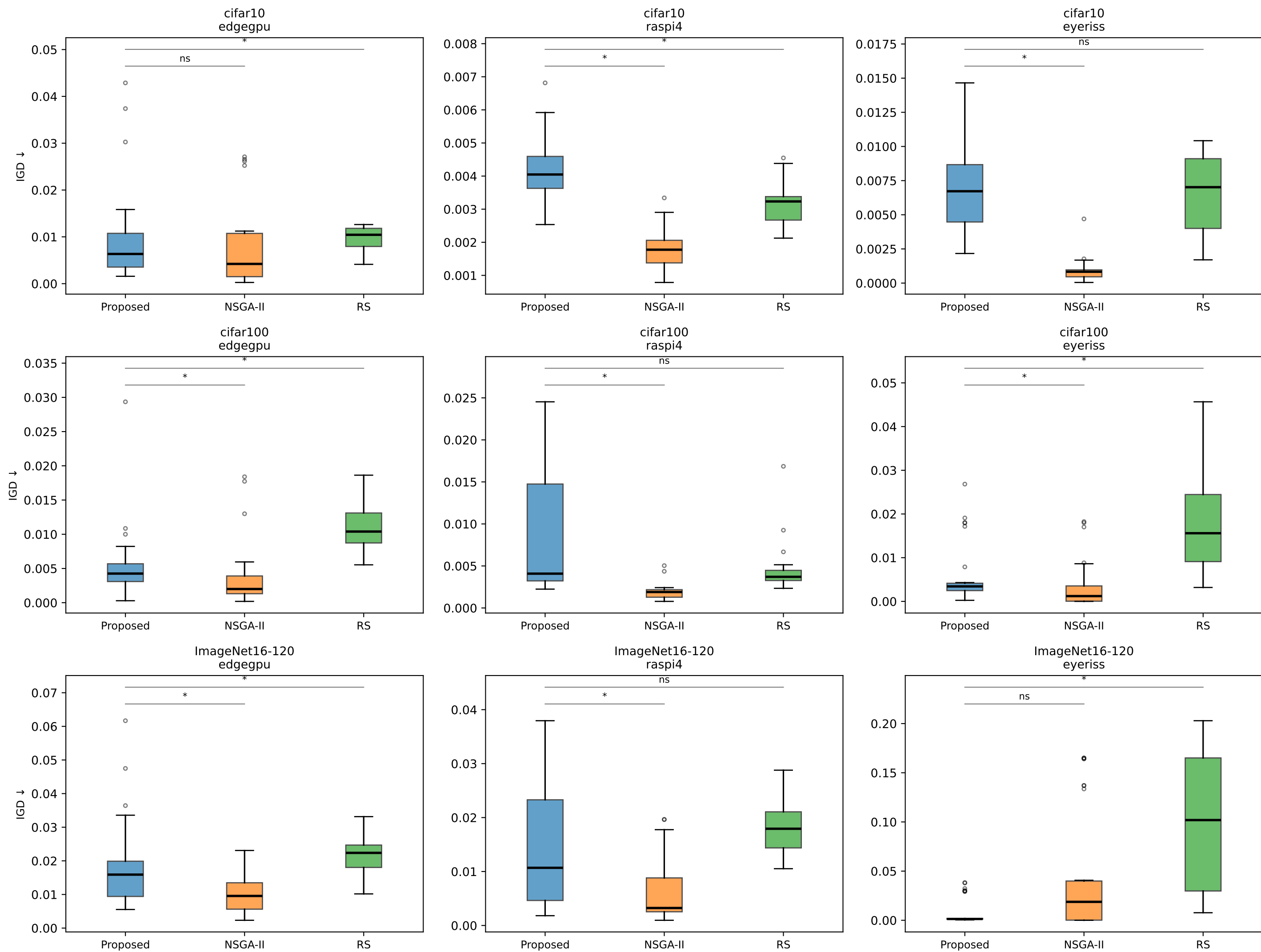
IGD ↓ Distribution Across 30 Seeds (normalised [0, 1]^2 objective space)
