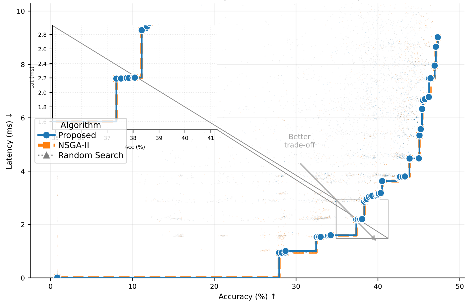
Pareto Front — ImageNet16-120 / Raspi4 Latency
