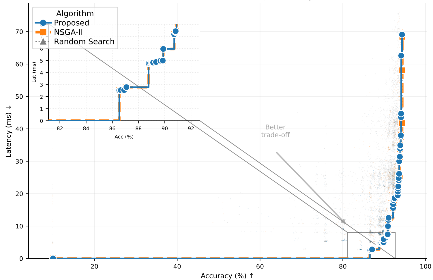
Pareto Front — cifar10 / Raspi4 Latency
