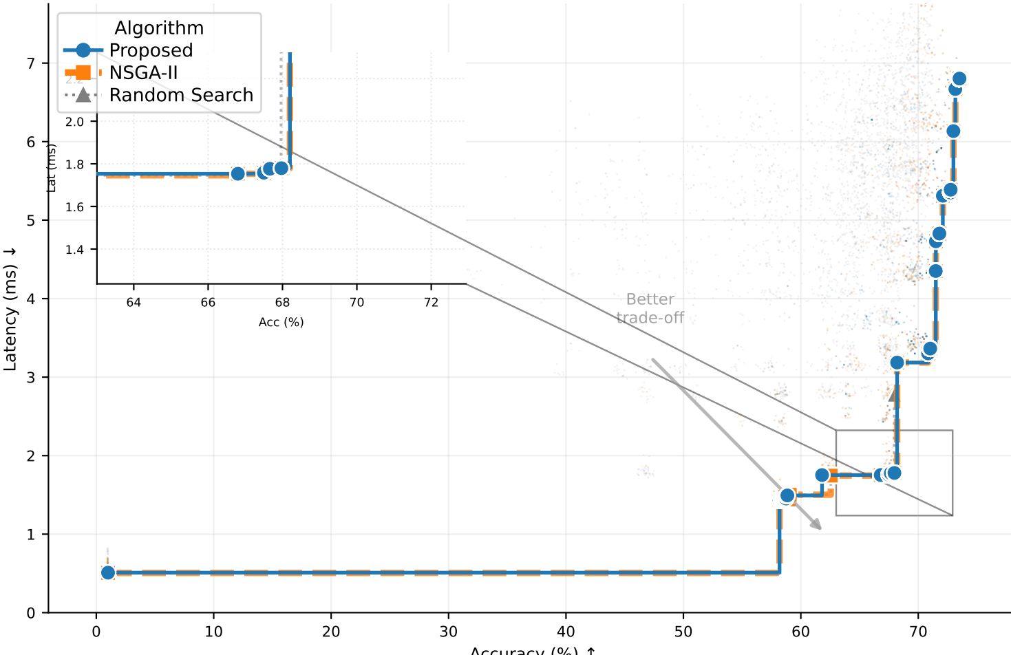
Pareto Front — cifar100 / Edgcpu Latency
