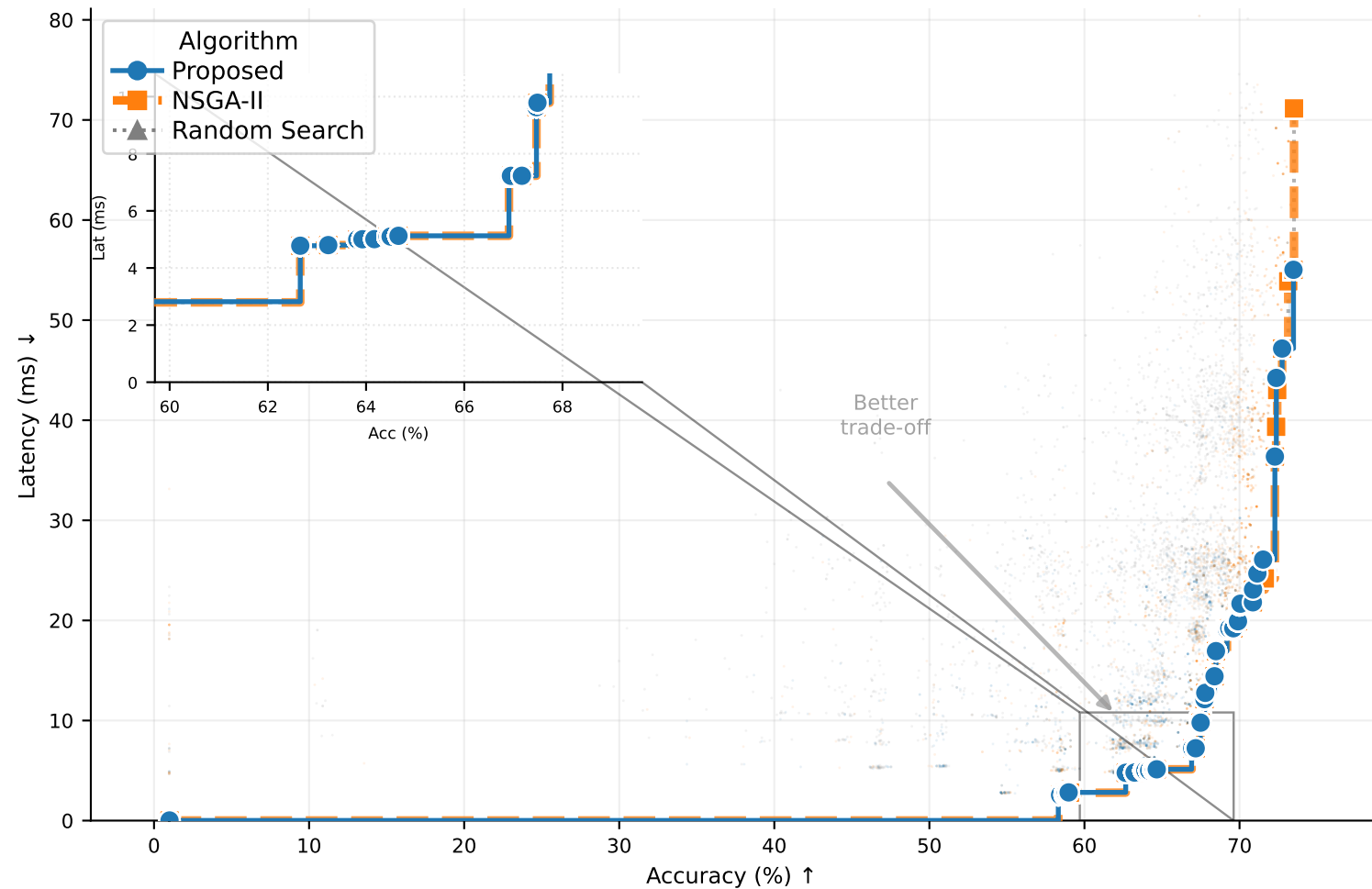
Pareto Front — cifar100 / Raspi4 Latency
