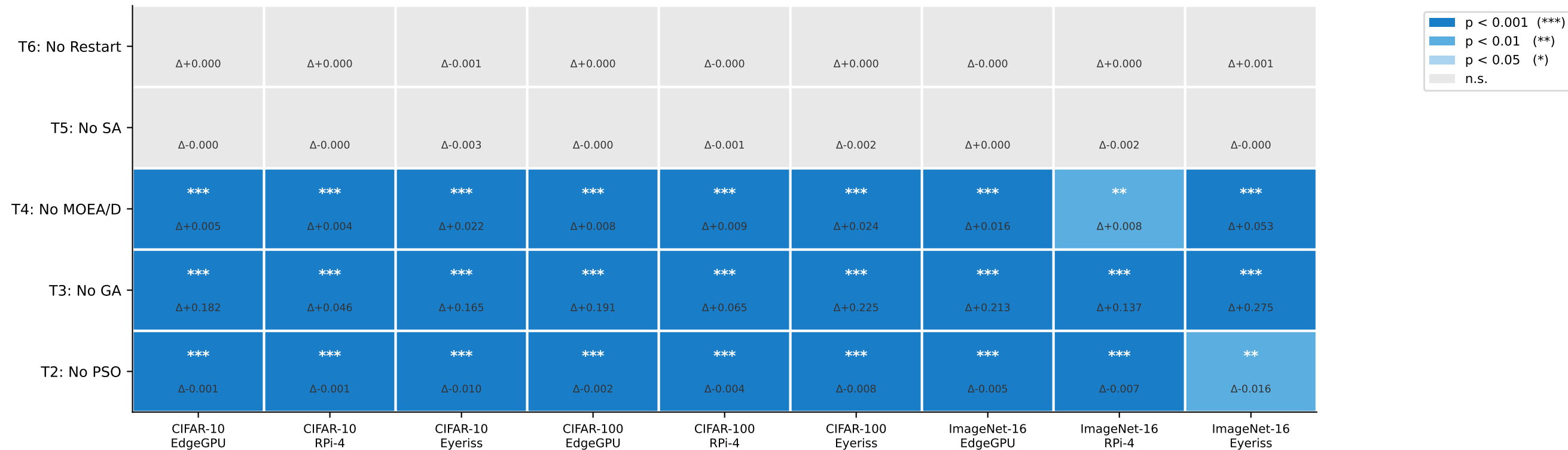
T1 Full Proposed vs Ablation Variants — Wilcoxon Significance Heatmap
