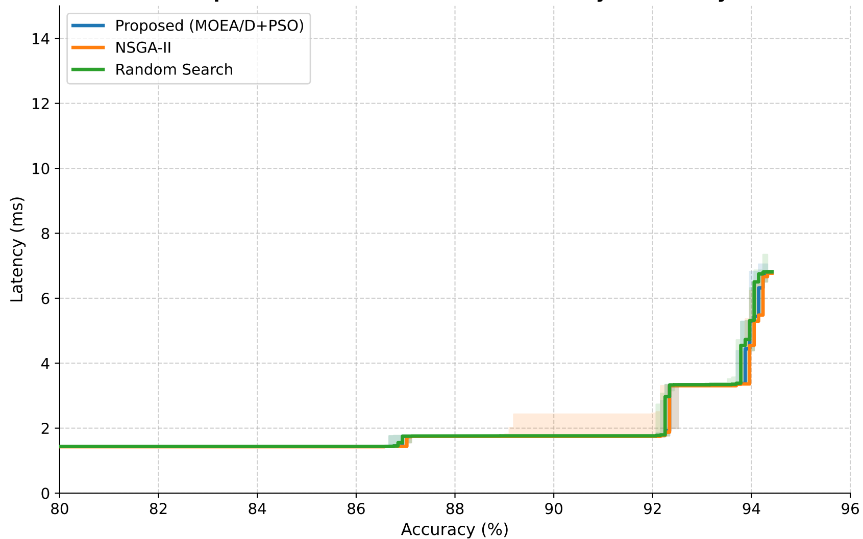
Empirical Attainment Surface: Accuracy vs Latency
