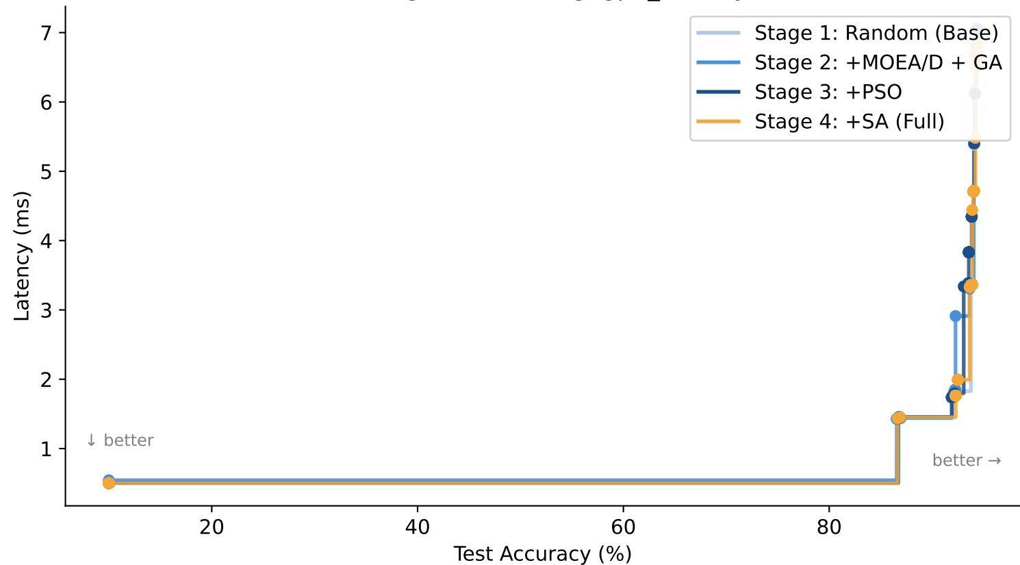
Waterfall Build-up: Pareto Fronts per Stage (seed=42, budget=2000, edgegpu_latency, cifar10)
