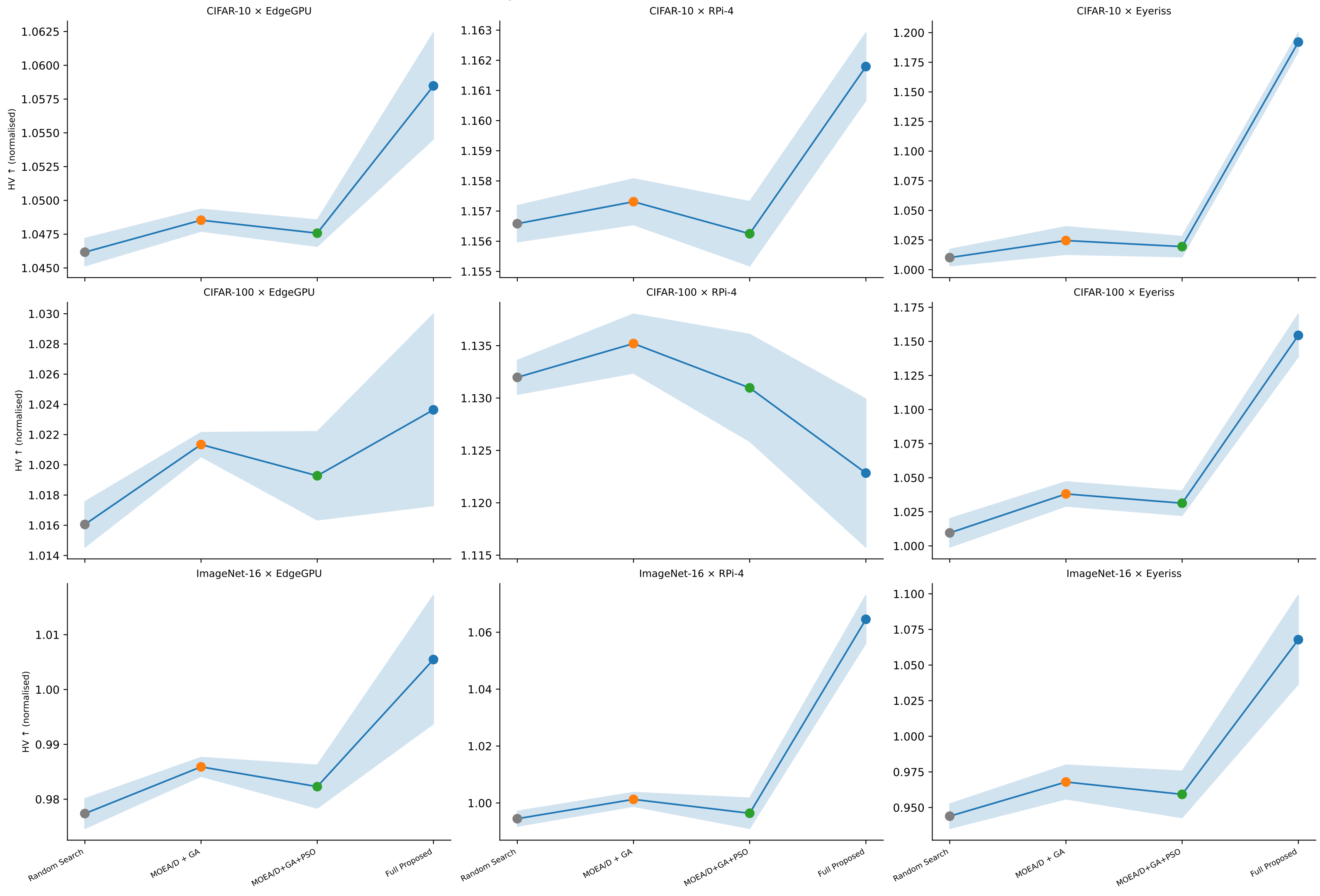
HV Progression (Waterfall, mean \pm std, 30 seeds) — 3 \times 3
