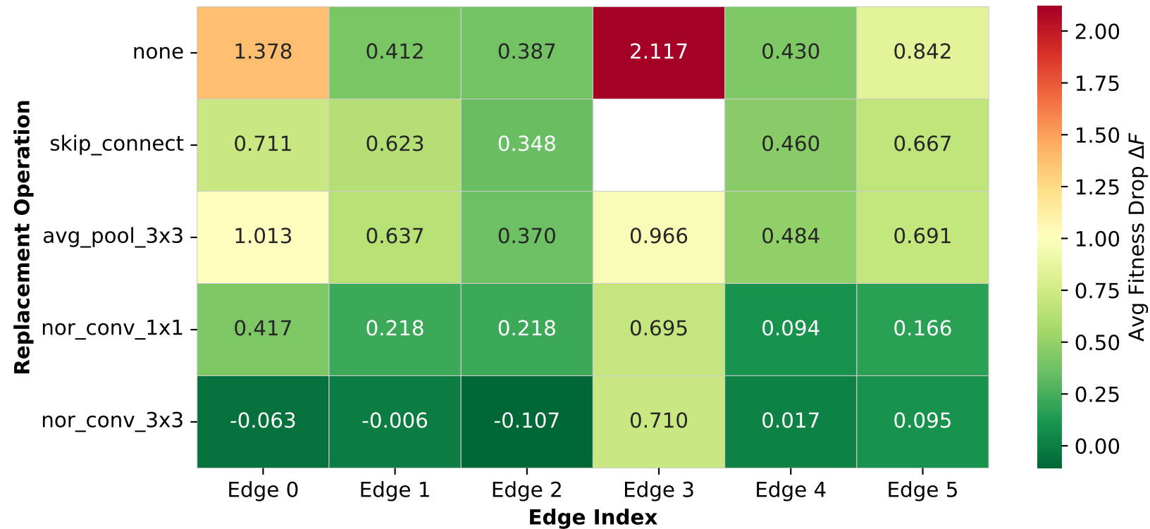
Epistasis Heatmap: Architecture Brittleness under Single-Edge Perturbation
