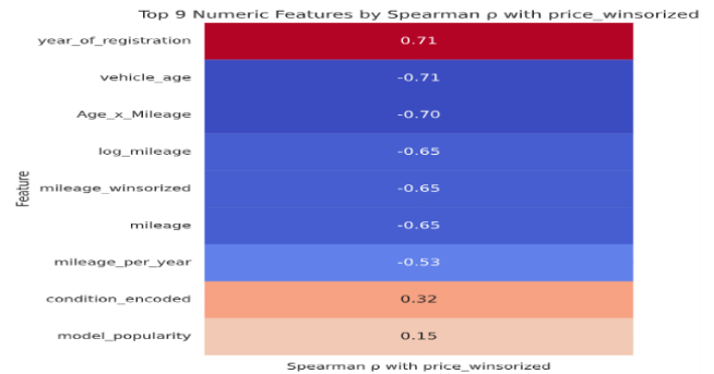
Figure 1.2 Spearman Correlation Heatmap of Numerical Features.
