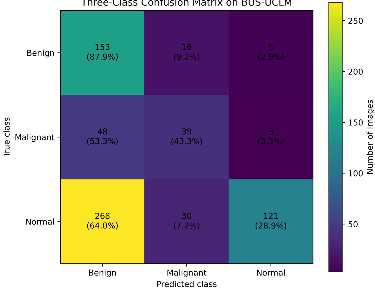
Three-Class Confusion Matrix on BUS-UCLM
