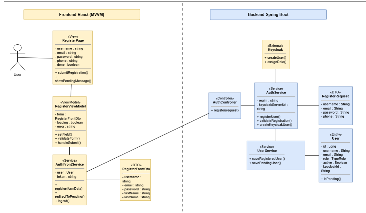
Figure 27: Design Class Diagram – Registration and Pending Access
