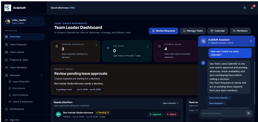
Figure 199: Assistant Platform Guidance Interface
