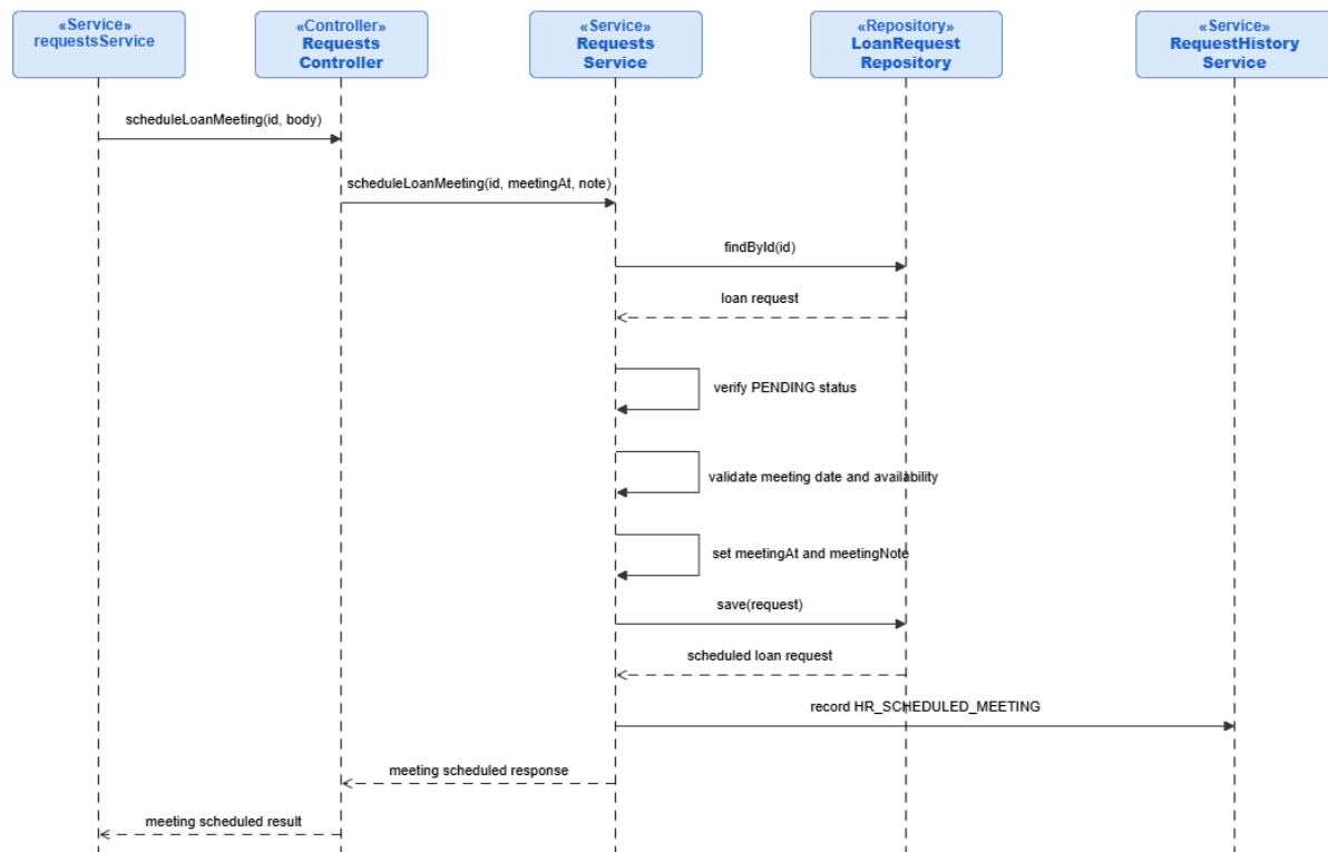
Figure 110: Conception Sequence Diagram – Loan Meeting Scheduling Backend
