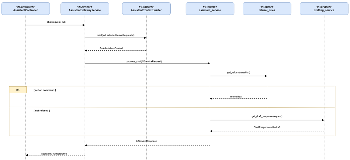
Figure 168: Conception Sequence Diagram – Assistant Request Drafting Backend
