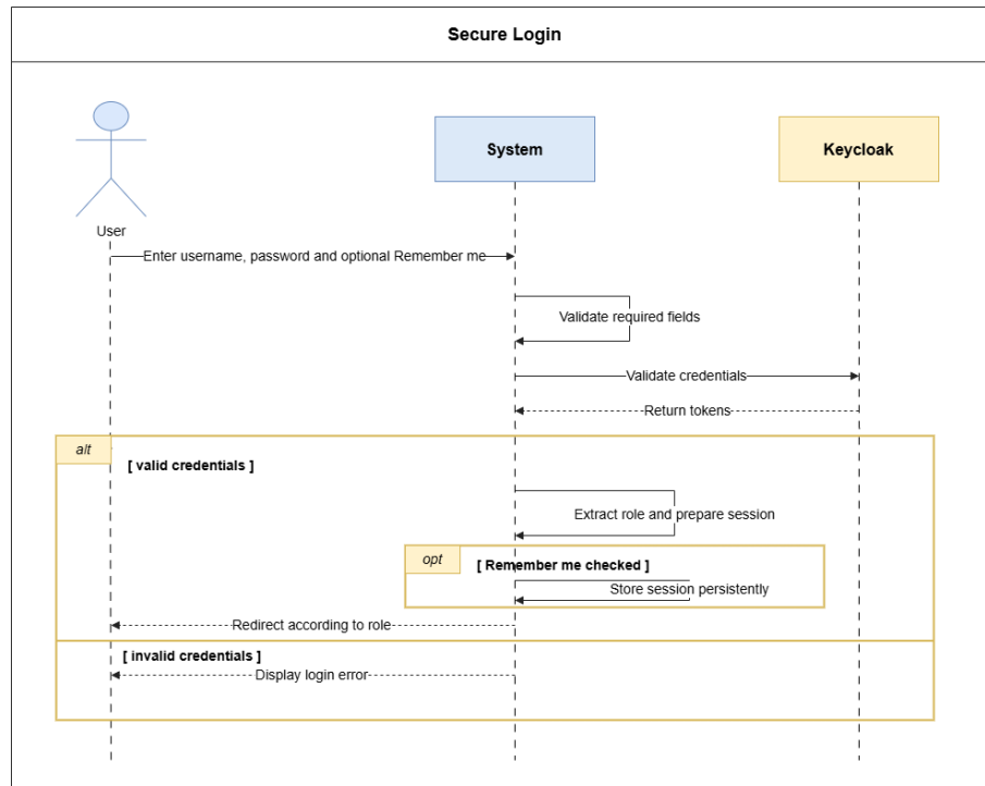
Figure 13: System Sequence Diagram – Secure Login
