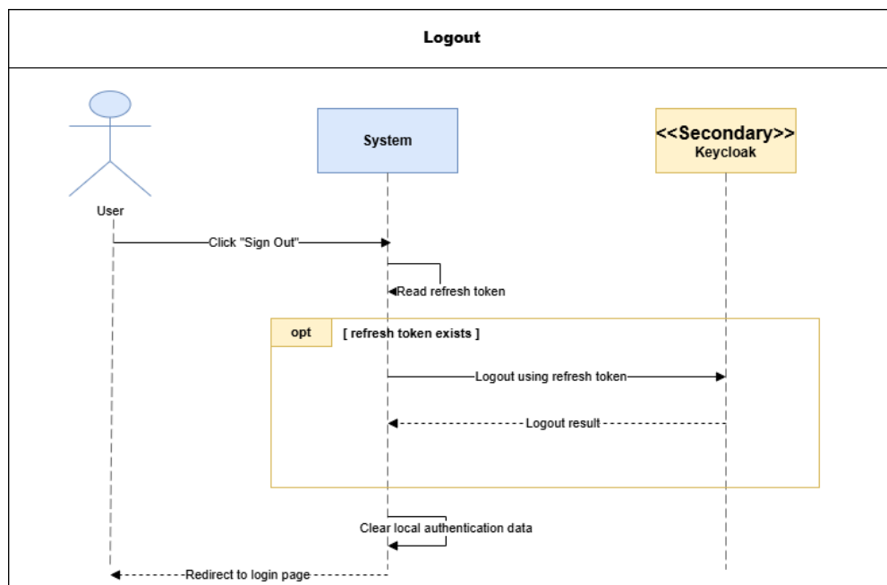
Figure 14: System Sequence Diagram – Logout
