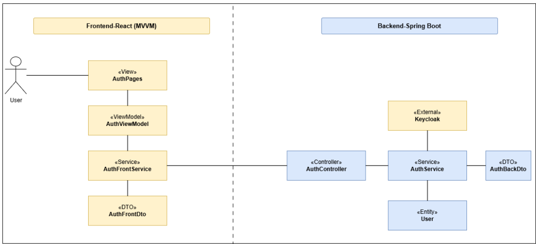
Figure 23: Participant Class Diagram – Authentication and Access Control
