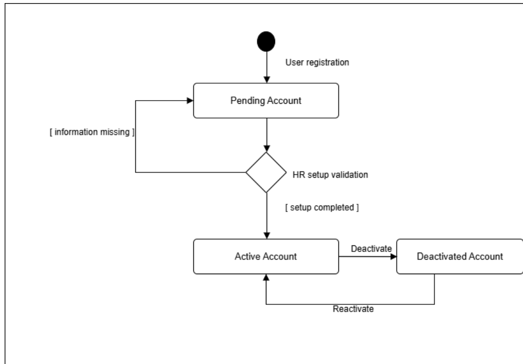
Figure 26: State Diagram – User Account Lifecycle
