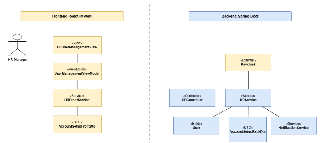
Figure 25: Participant Class Diagram – HR Account Management
