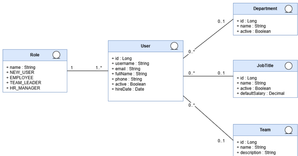
Figure 22: Domain Model – Sprint 1 Access and Account Management
