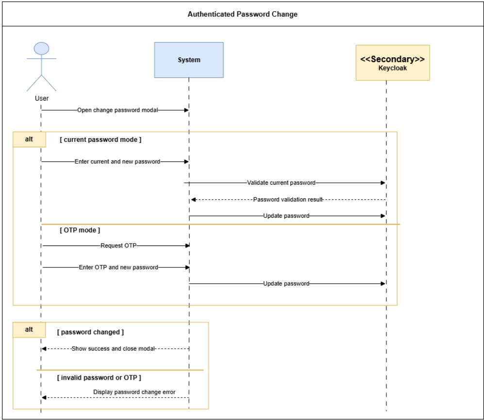
Figure 18: System Sequence Diagram – Authenticated Password Change
