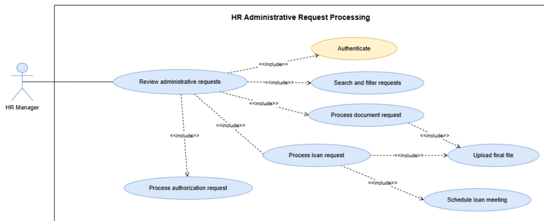
Figure 72: Use Case Diagram – HR Administrative Request Processing
