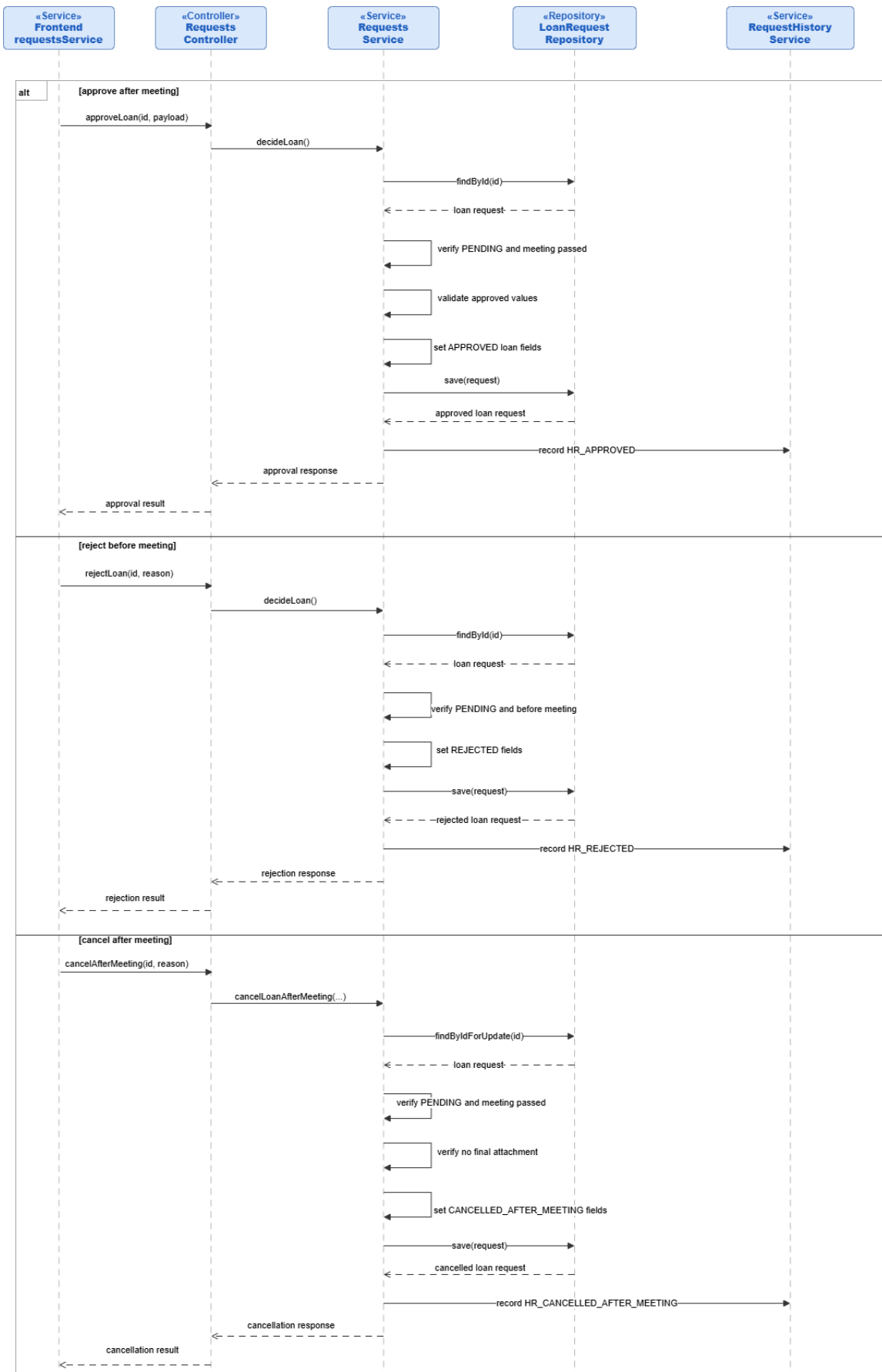
Figure 100: Conception Sequence Diagram – Loan Request Decision Backend
