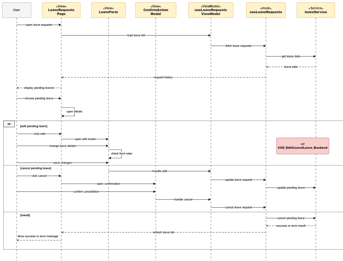
Figure 64: Conception Sequence Diagram – Edit or Cancel Pending Leave Frontend
