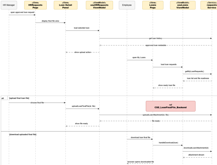
Figure 101: Conception Sequence Diagram – Loan Final File Delivery Frontend
