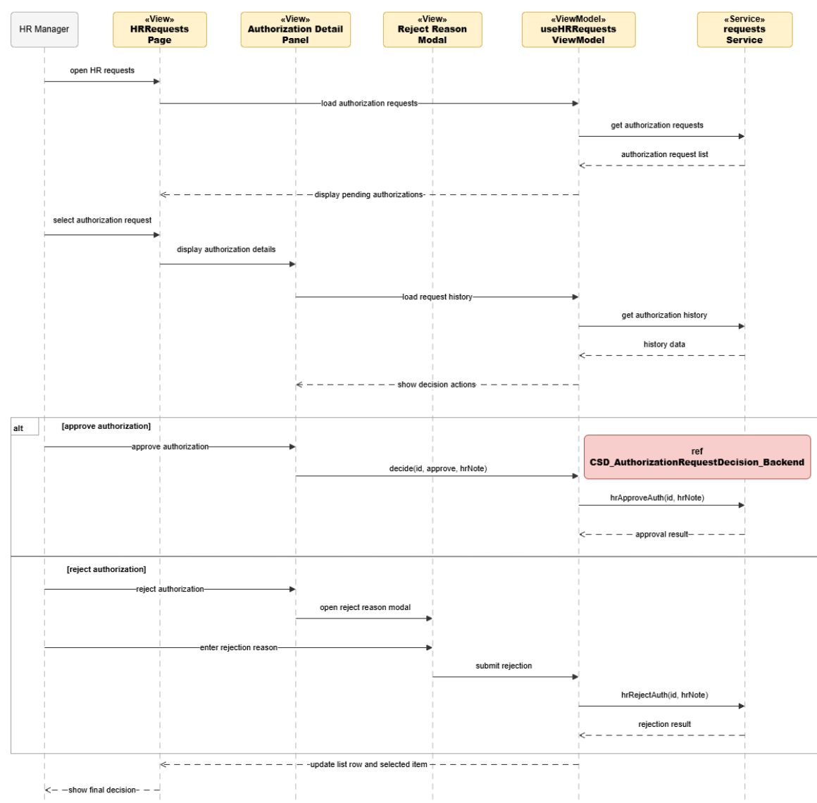
Figure 105: Conception Sequence Diagram – Authorization Request Decision Frontend
