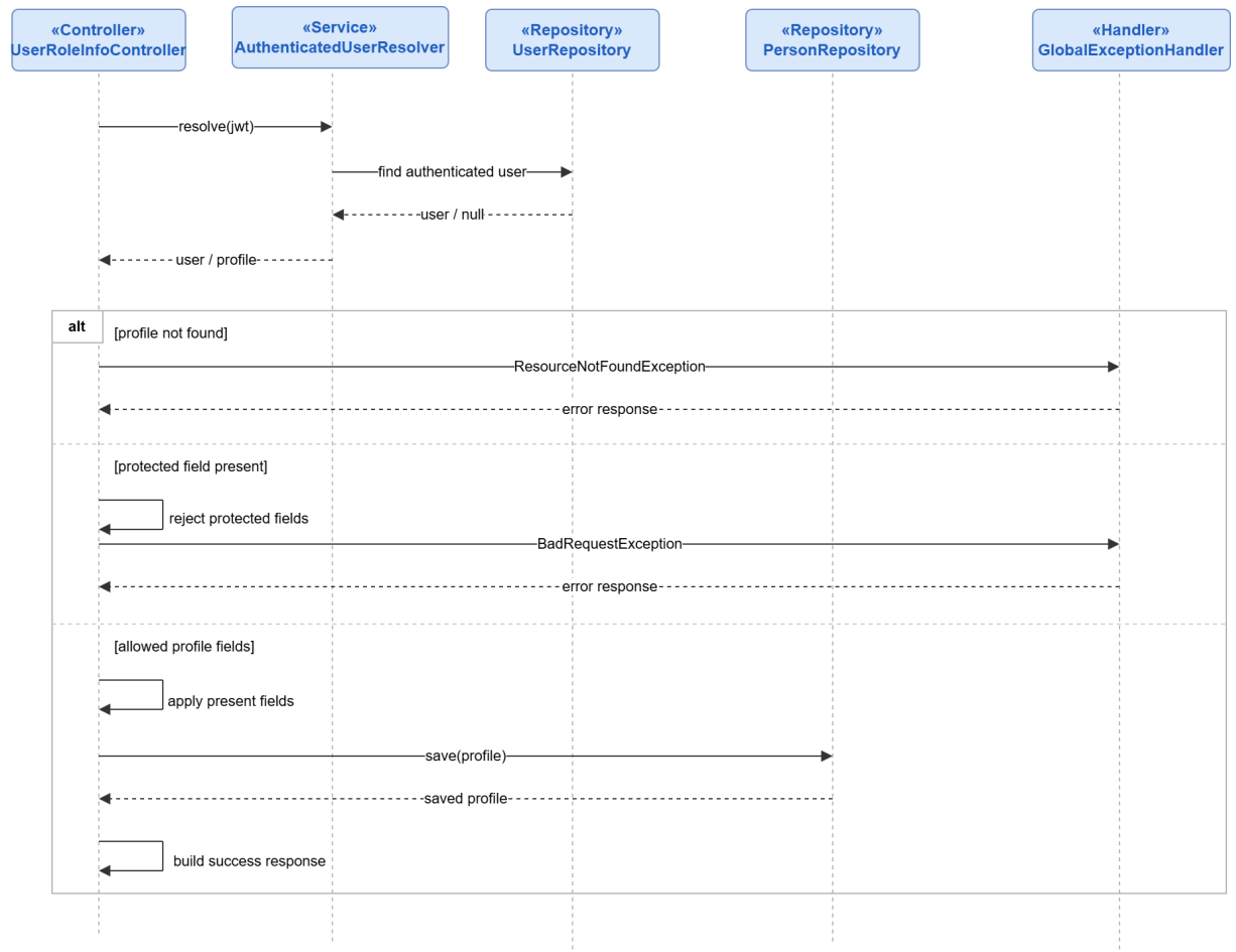
Figure 39: Conception Sequence Diagram – Profile Update Backend
