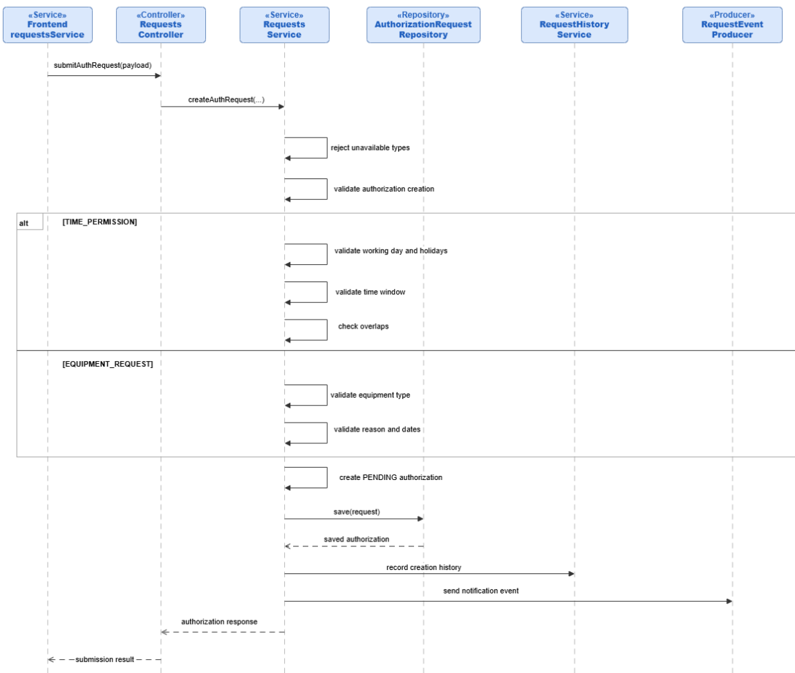
Figure 104: Conception Sequence Diagram – Authorization Request Submission Backend
