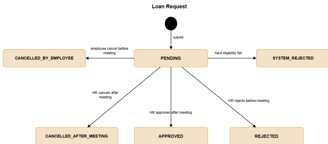
Figure 85: State Diagram – Loan Request Lifecycle
