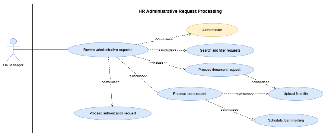
Figure 72: Use Case Diagram – HR Administrative Request Processing
