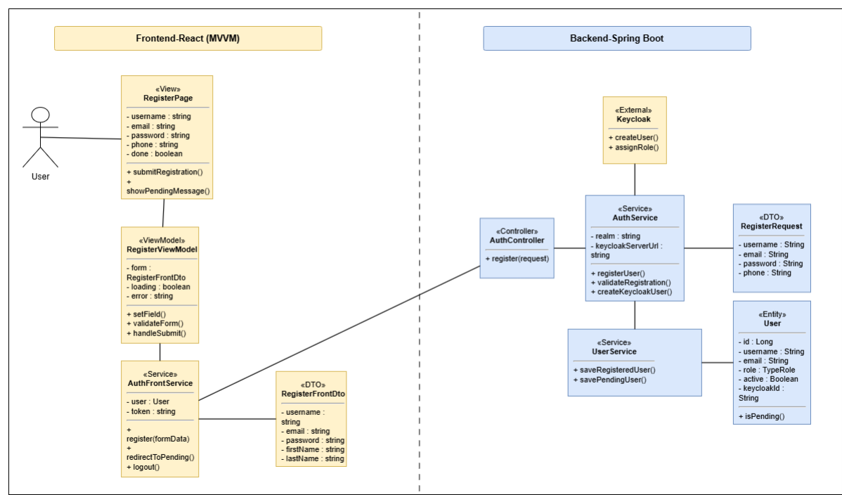
Figure 27: Design Class Diagram – Registration and Pending Access
