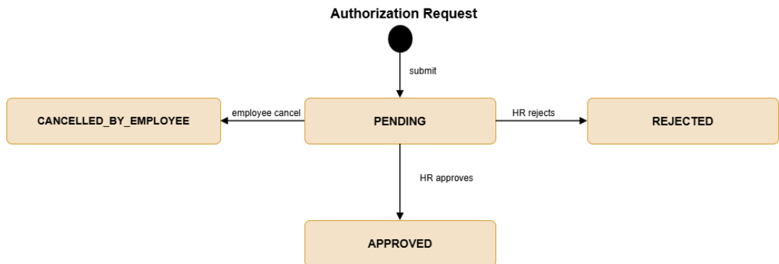
Figure 86: State Diagram – Authorization Request Lifecycle
