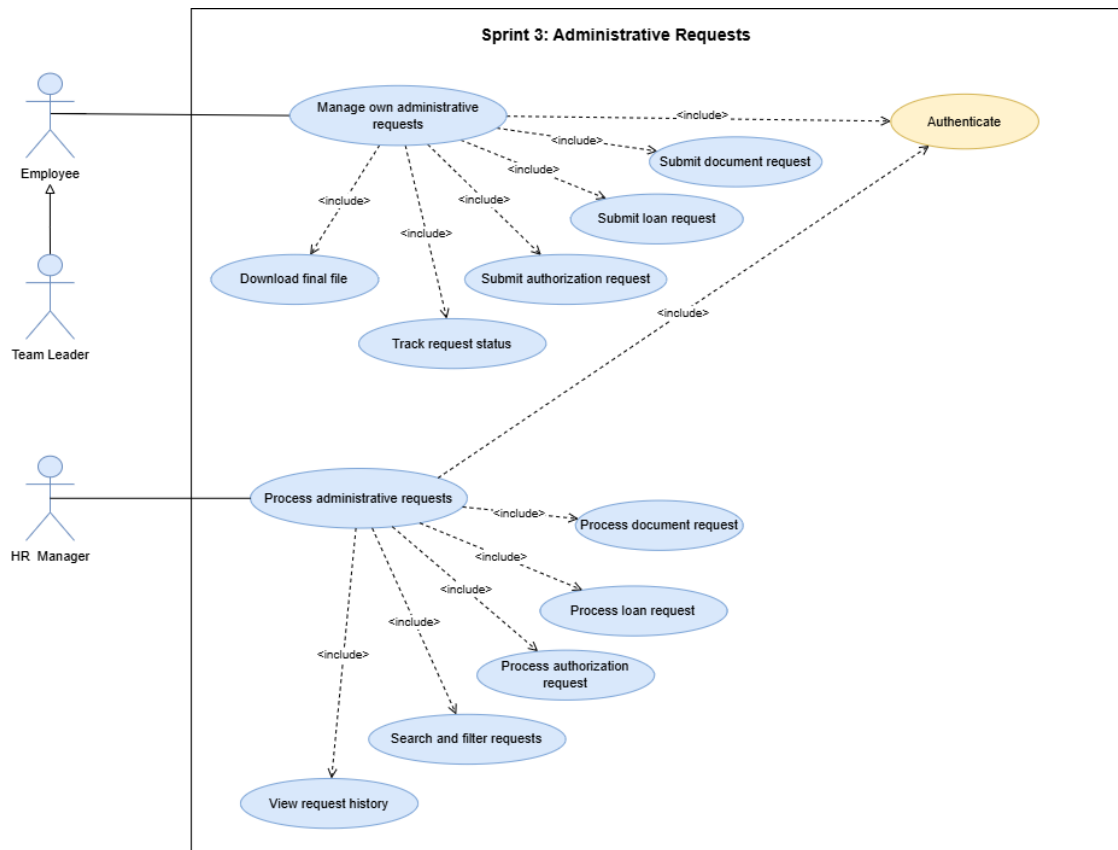
Figure 71: Use Case Diagram – Sprint 3 Administrative Requests
