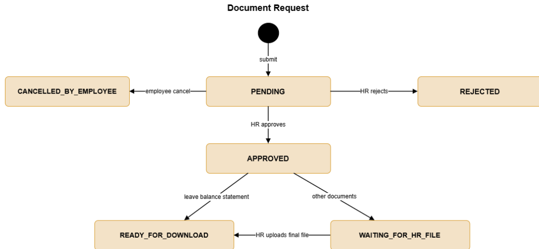
Figure 84: State Diagram – Document Request Lifecycle
