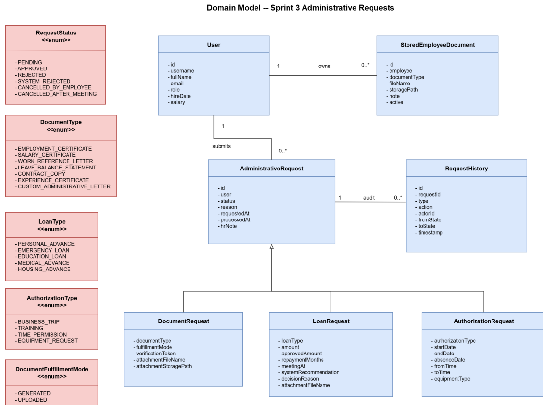
Figure 79: Domain Model – Sprint 3 Administrative Requests
