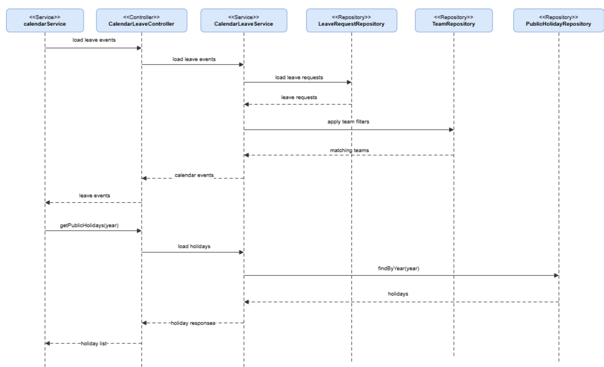
Figure 152: Conception Sequence Diagram – HR Leave Calendar Backend
