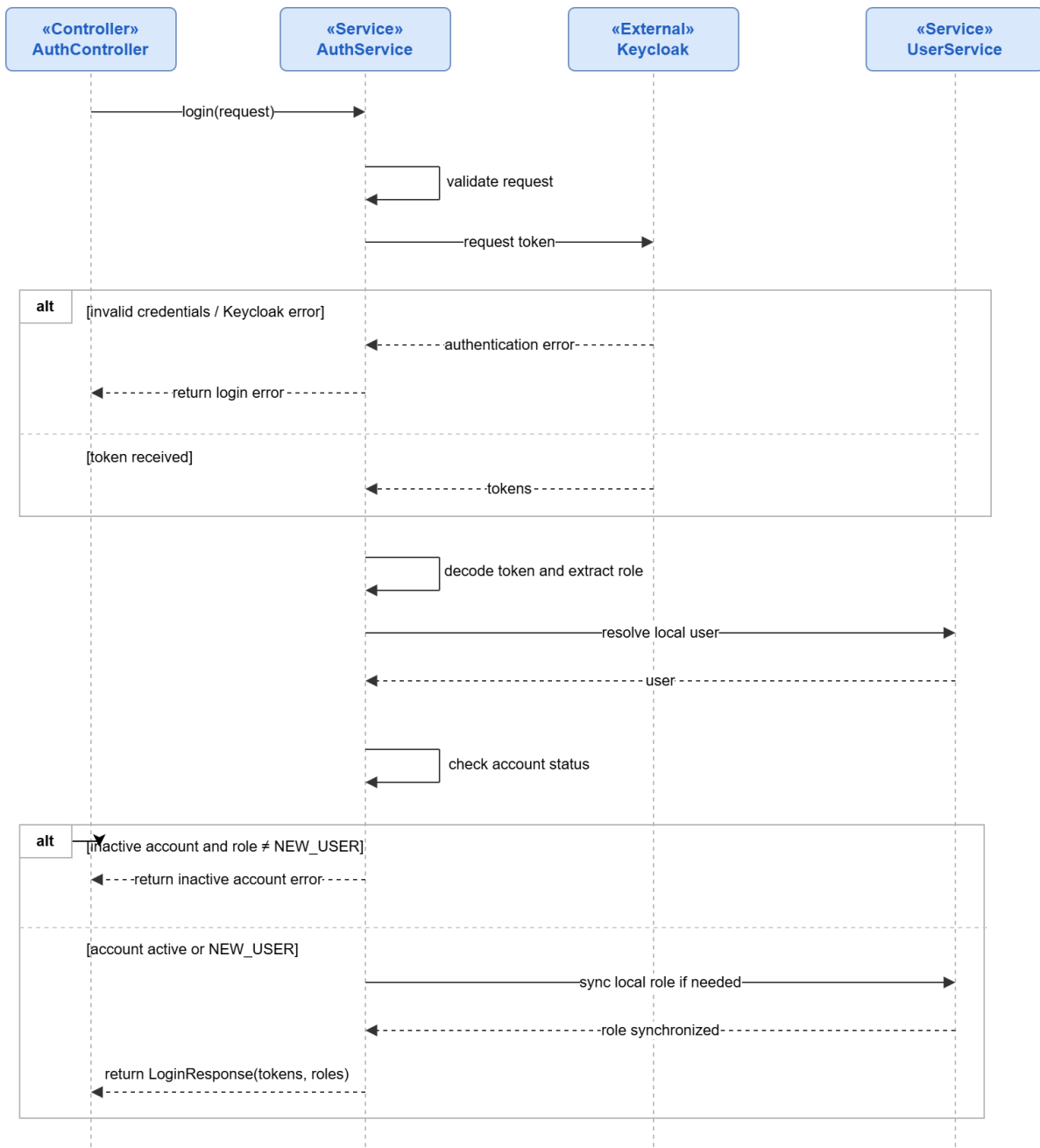
Figure 33: Conception Sequence Diagram – Secure Login Backend
