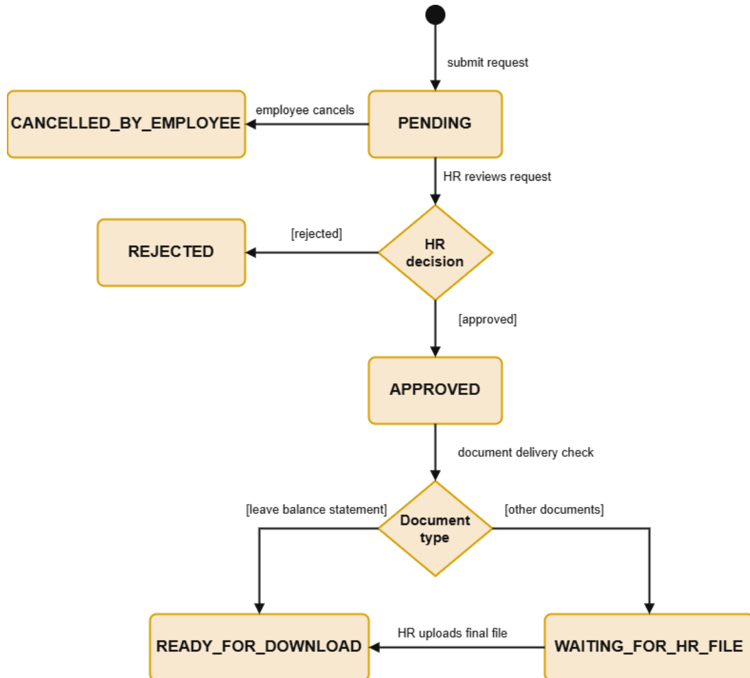
Figure 96: State Diagram – Document Request Lifecycle
