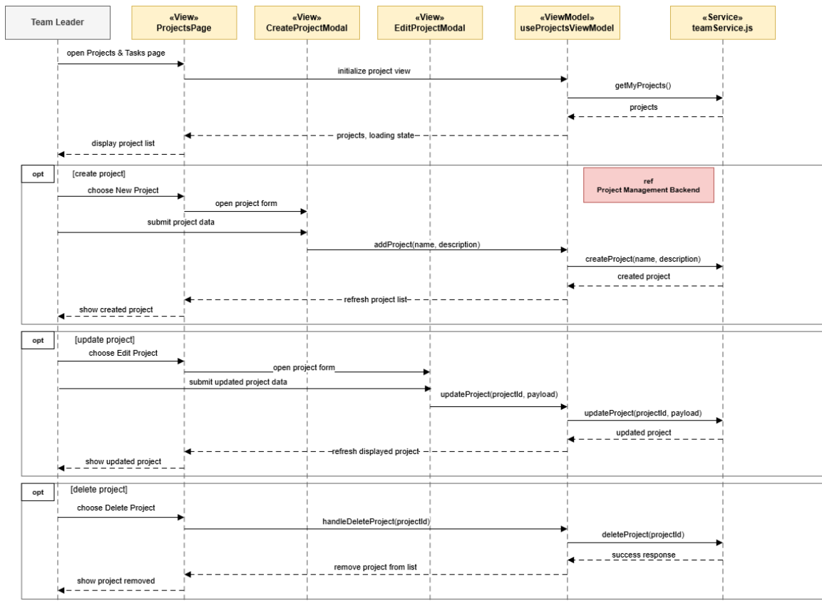
Figure 175: Conception Sequence Diagram – Project Management Frontend
