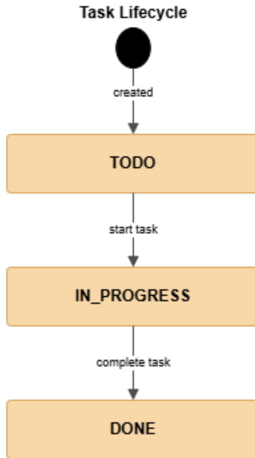
Figure 168: State Diagram – Task Lifecycle
