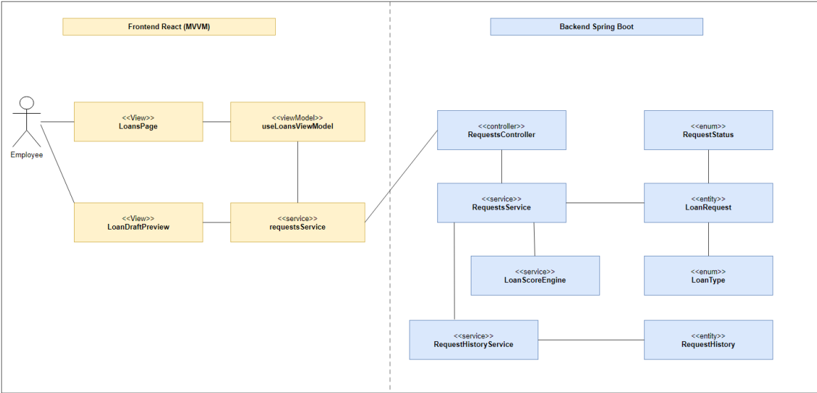
Figure 93: Participant Class Diagram – Loan Request Management
