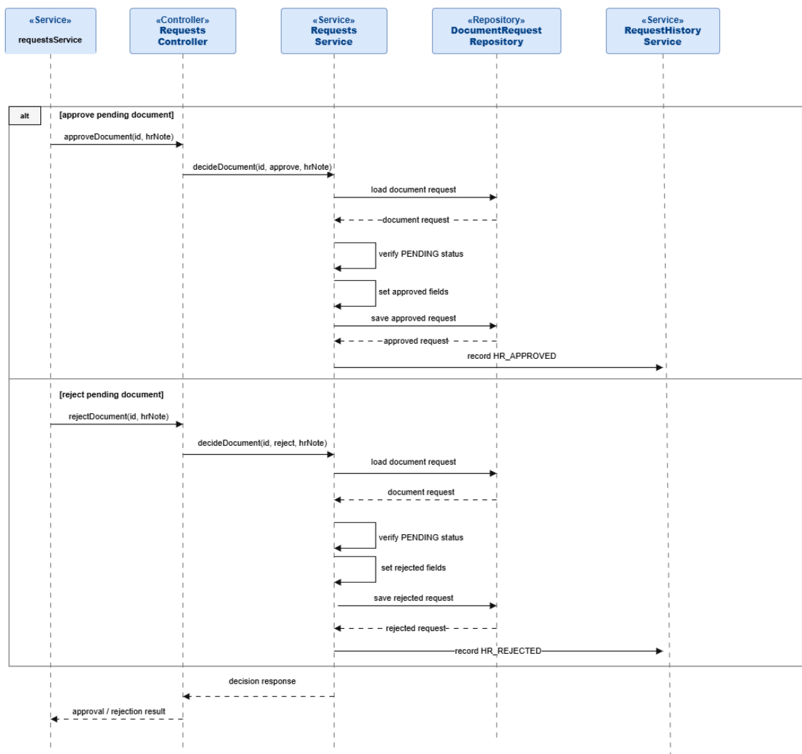
Figure 104: Conception Sequence Diagram – Document Request Decision Backend
