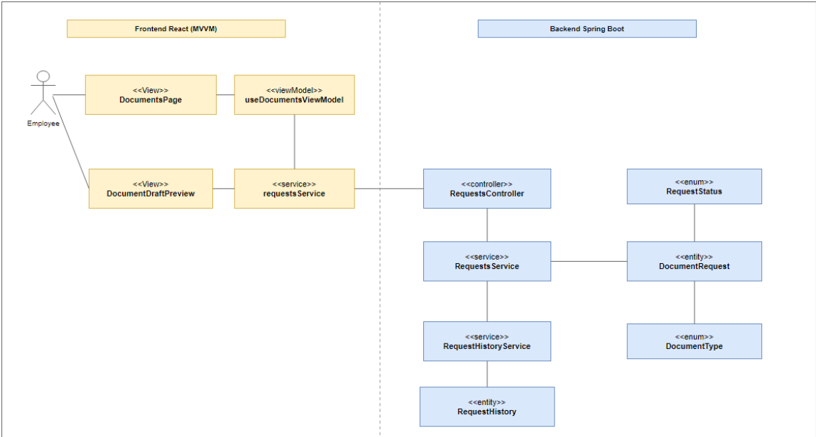
Figure 92: Participant Class Diagram – Document Request Management
