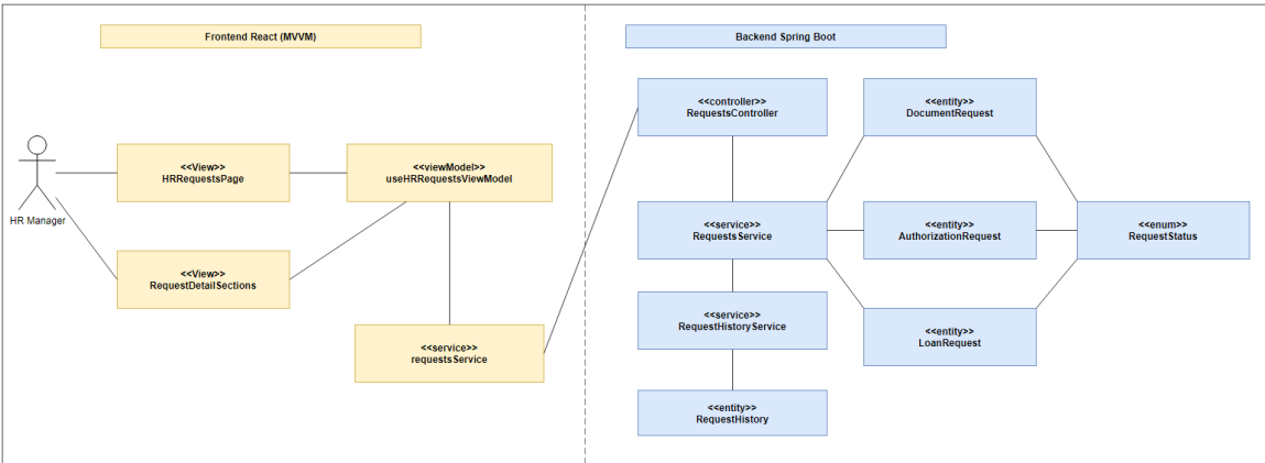
Figure 95: Participant Class Diagram – HR Request Processing
