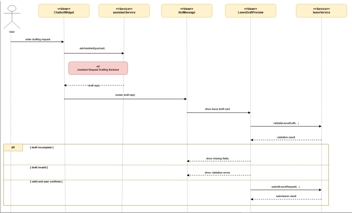
Figure 195: Conception Sequence Diagram – Assistant Request Drafting Frontend
