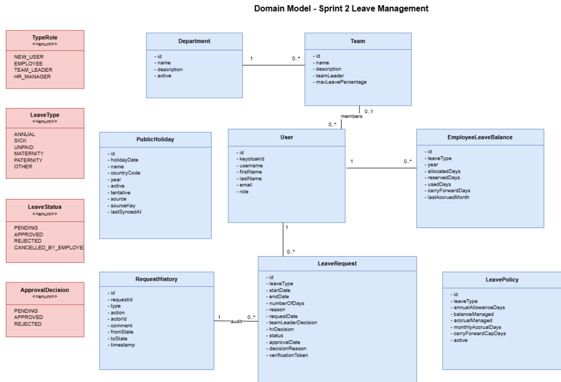
Figure 60: Domain Model – Sprint 2 Leave Management
