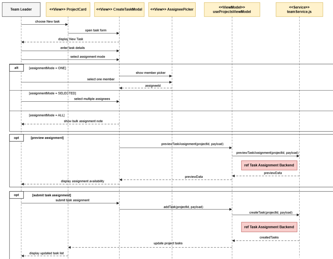
Figure 177: Conception Sequence Diagram – Task Assignment Frontend
