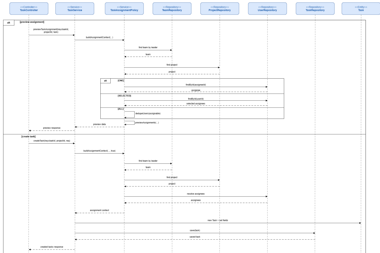
Figure 178: Conception Sequence Diagram – Task Assignment Backend
