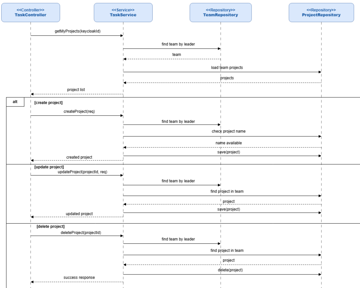
Figure 176: Conception Sequence Diagram – Project Management Backend
