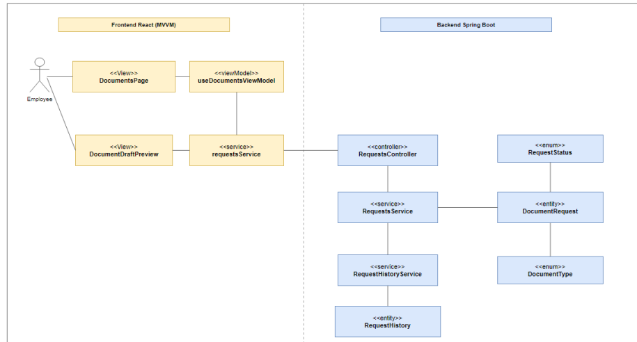
Figure 92: Participant Class Diagram – Document Request Management
