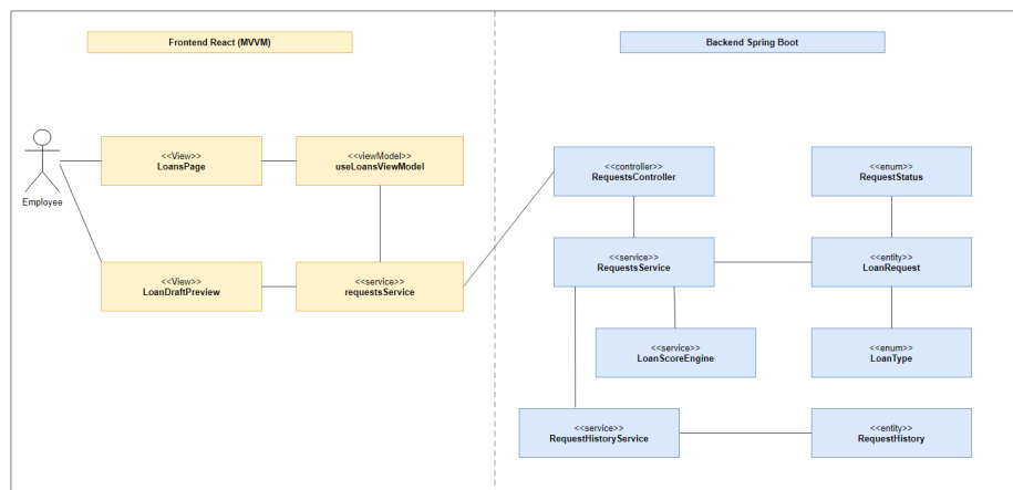
Figure 93: Participant Class Diagram – Loan Request Management
