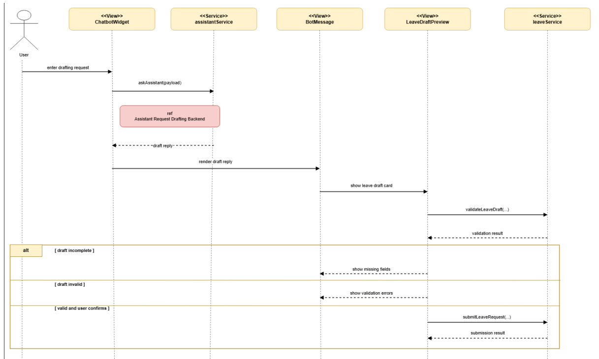
Figure 130: Conception Sequence Diagram – Assistant Request Drafting Frontend
