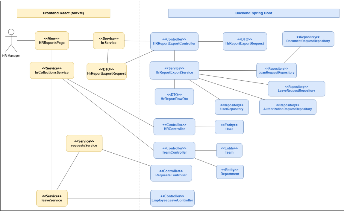
Figure 106: Participant Class Diagram – HR Reports and Export
