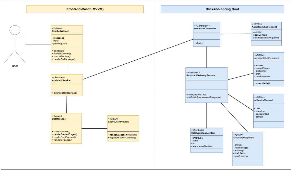
Figure 127: Design Class Diagram – Assistant Gateway and Safe Context
