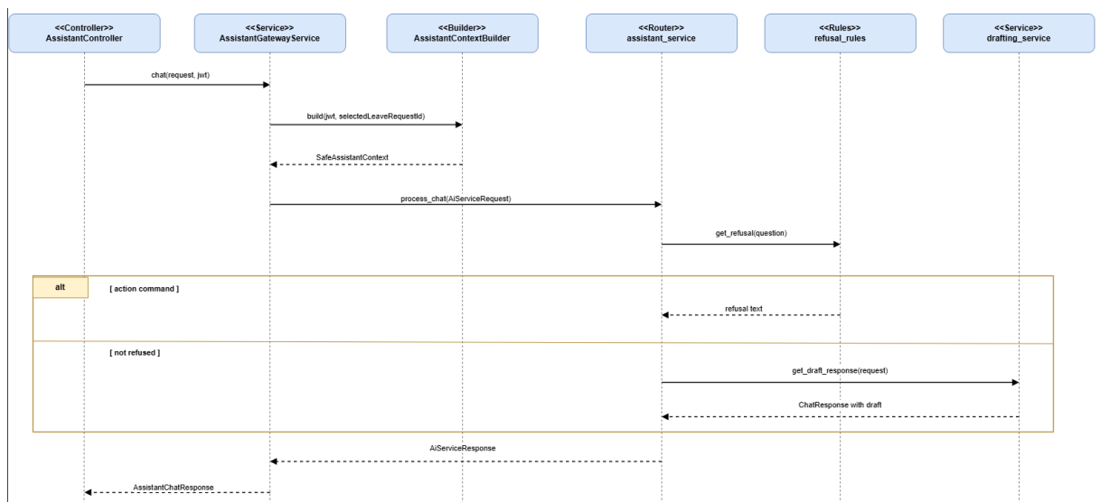
Figure 131: Conception Sequence Diagram – Assistant Request Drafting Backend
