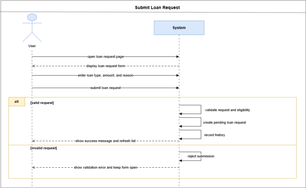
Figure 85: System Sequence Diagram – Submit Loan Request
