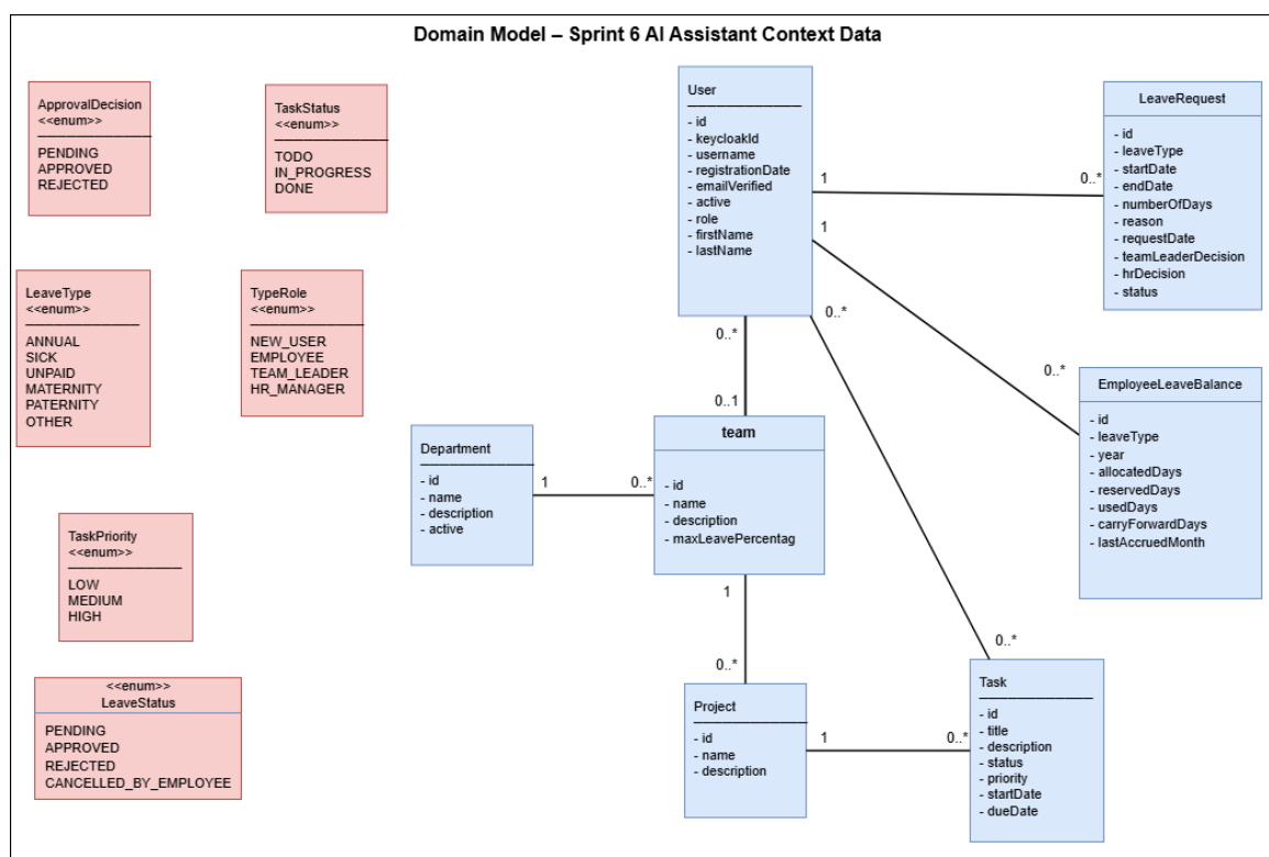
Figure 125: Domain Model – Sprint 6 AI Assistant Context Data
