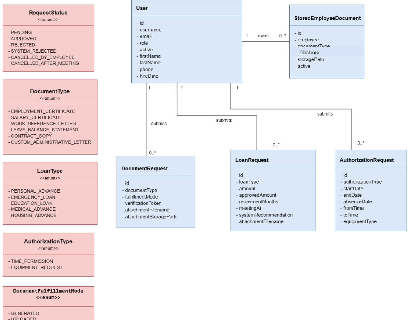
Figure 82: Domain Model – Sprint 3 Administrative Requests
