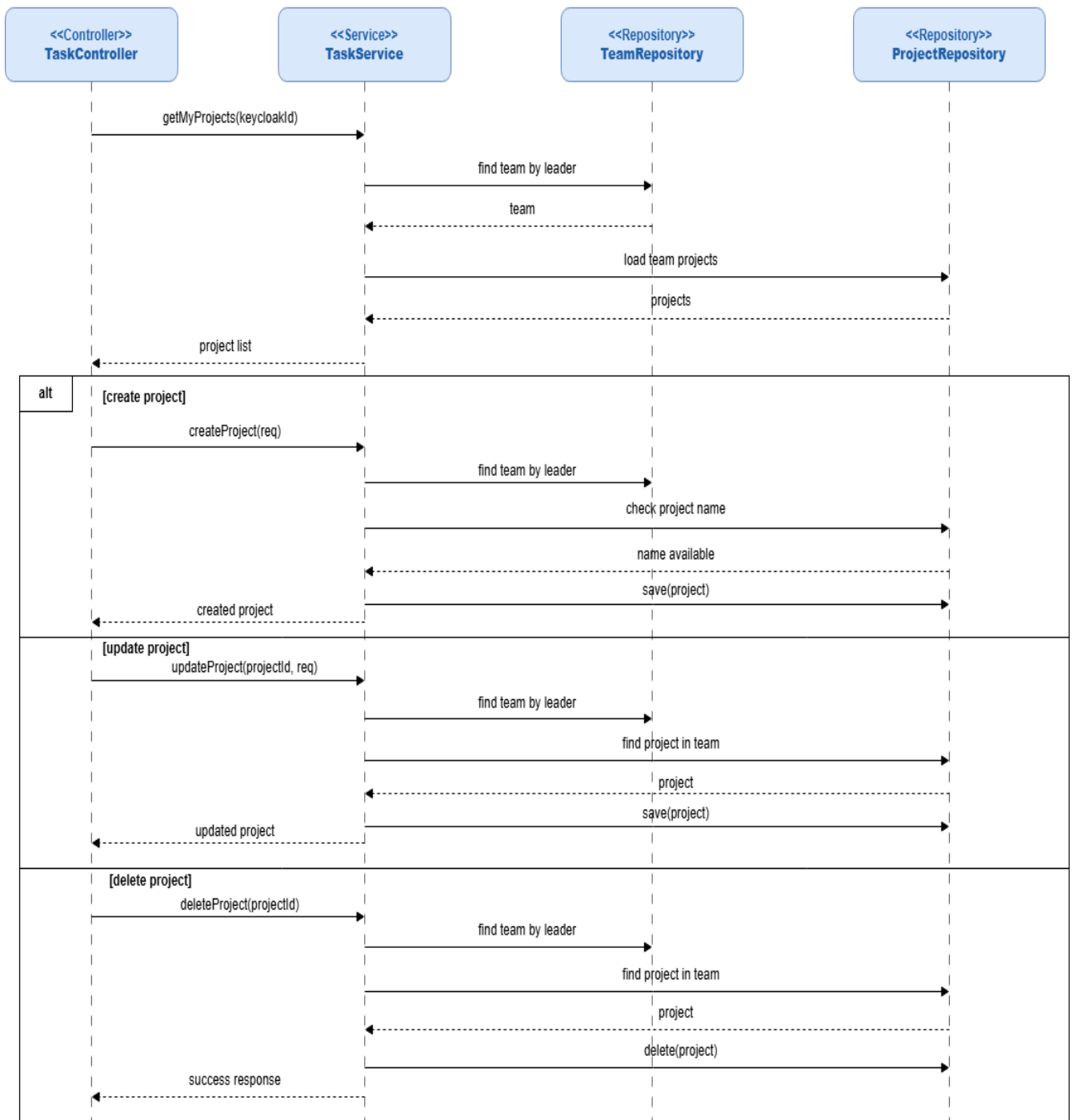
Figure 111: Conception Sequence Diagram – Project Management Backend
