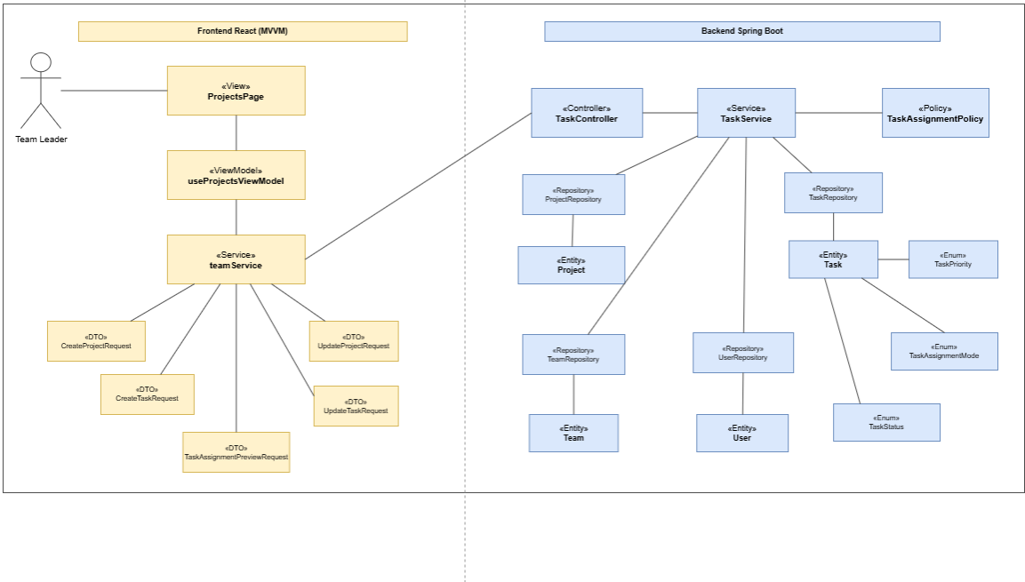
Figure 104: Participant Class Diagram – Team Leader Project and Task Management
