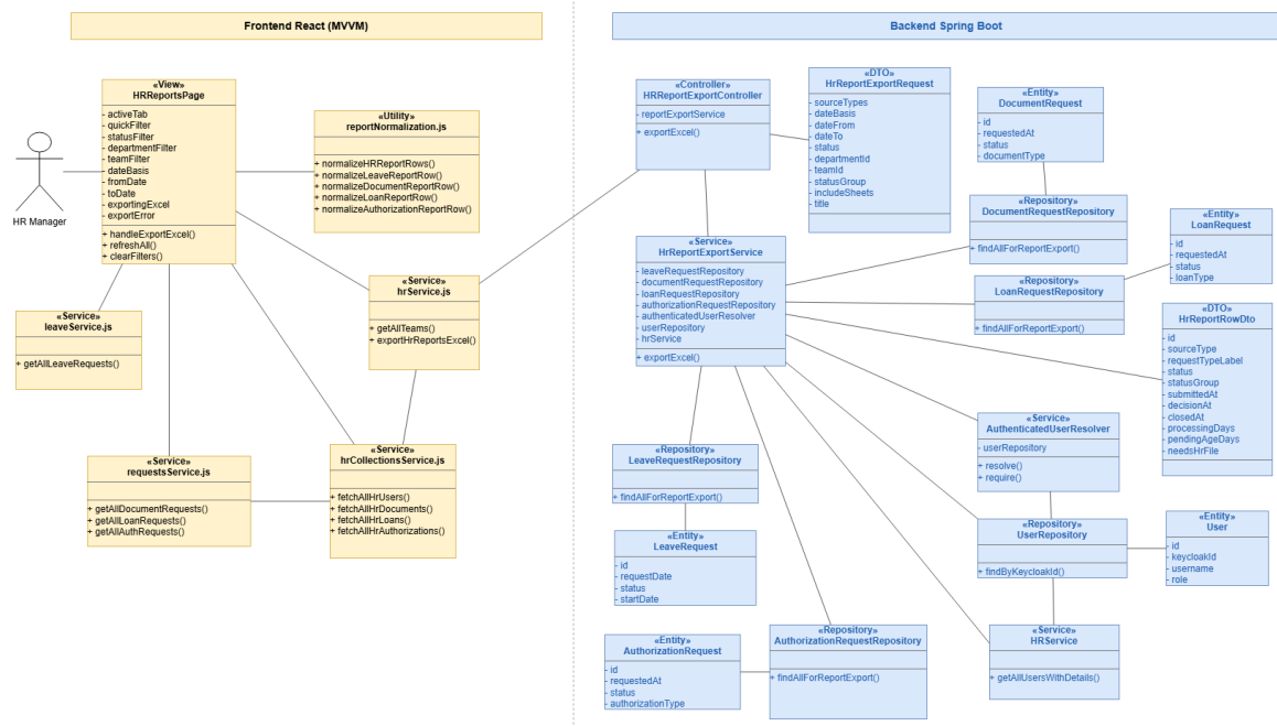
Figure 109: Design Class Diagram – HR Reports and Excel Export
