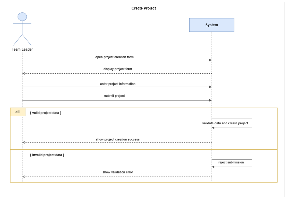
Figure 99: System Sequence Diagram – Create Project
