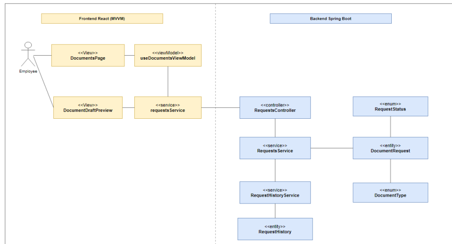
Figure 83: Participant Class Diagram – Document Request Management
