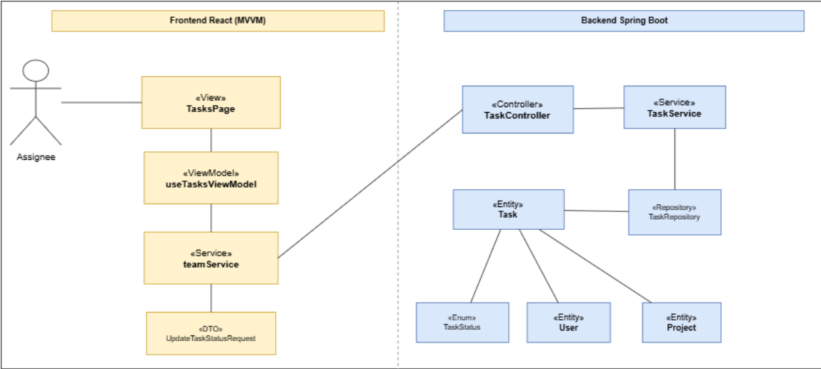
Figure 105: Participant Class Diagram – Task Status Update
