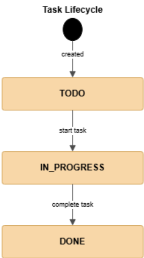
Figure 103: State Diagram – Task Lifecycle
