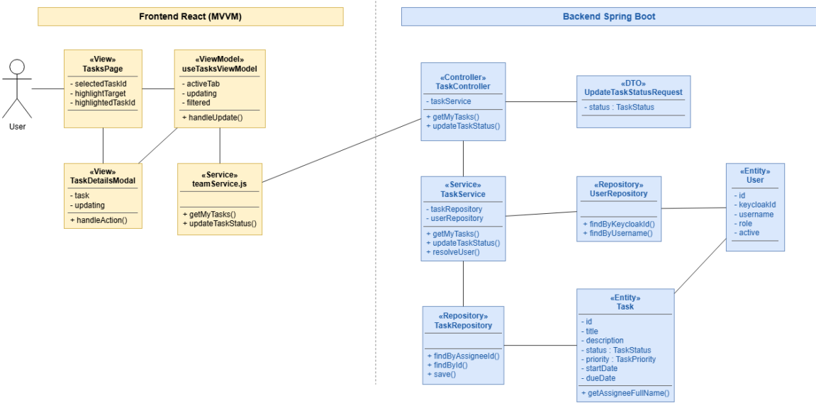
Figure 108: Design Class Diagram – Task Status Update
