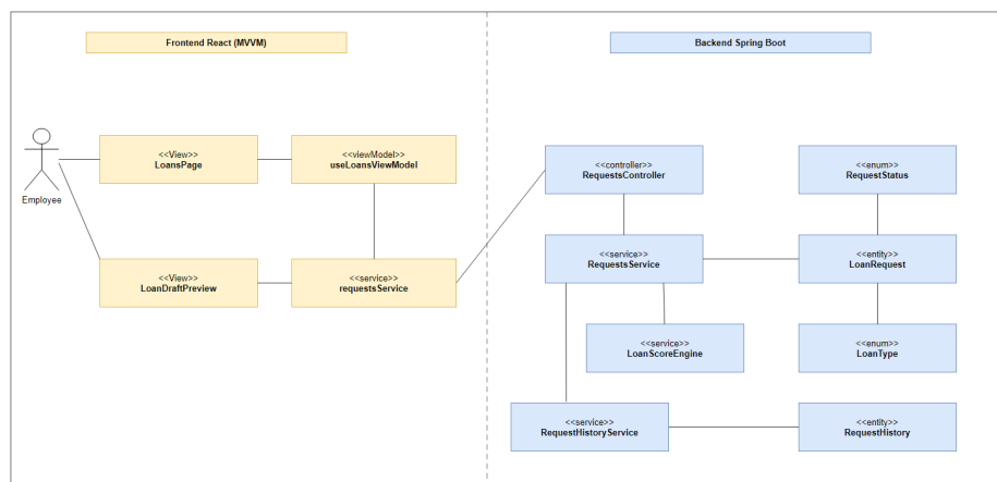
Figure 84: Participant Class Diagram – Loan Request Management
