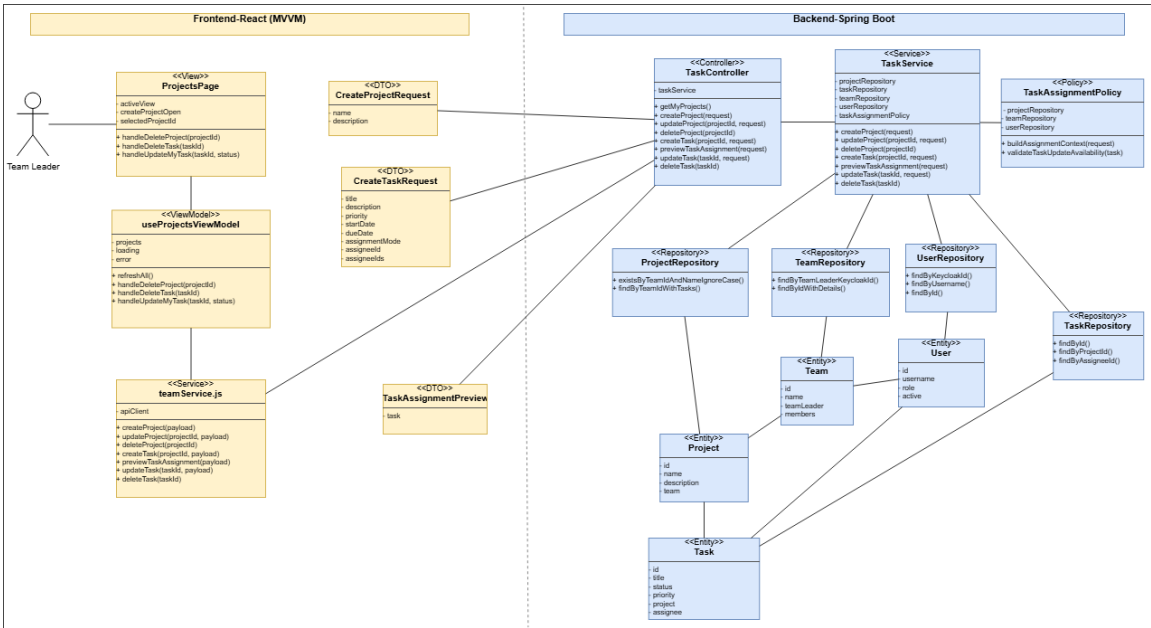
Figure 107: Design Class Diagram – Team Leader Project and Task Management
