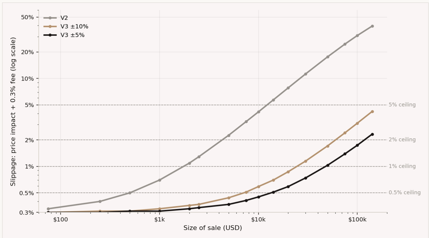
Figure 8. Slippage against sale size, USD 1m pool, three designs
