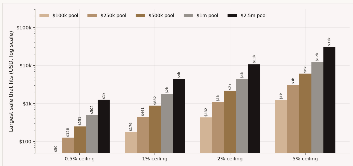
Figure 2. Largest sale inside each ceiling, V2 pool
