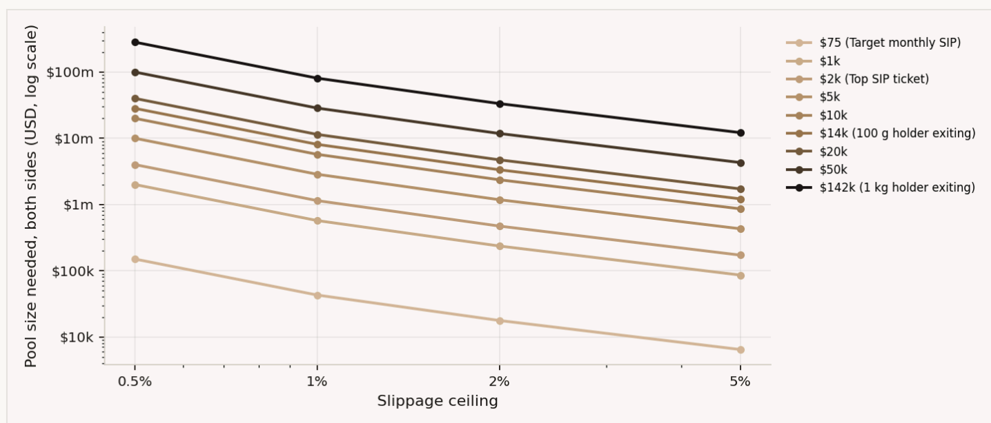
Figure 3. Pool size needed against slippage ceiling, V2, one line per trade size
