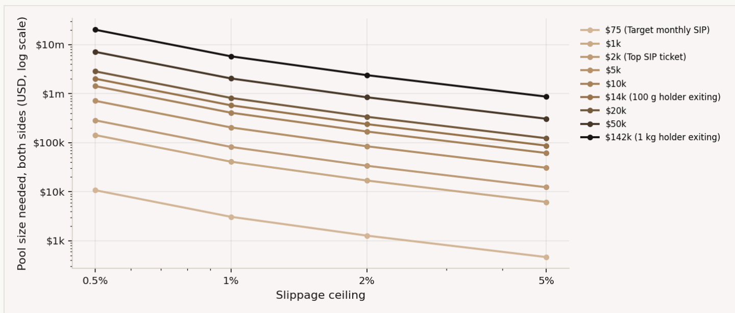
Figure 7. Pool size needed against slippage ceiling, V3 \pm 10\% , one line per trade size
