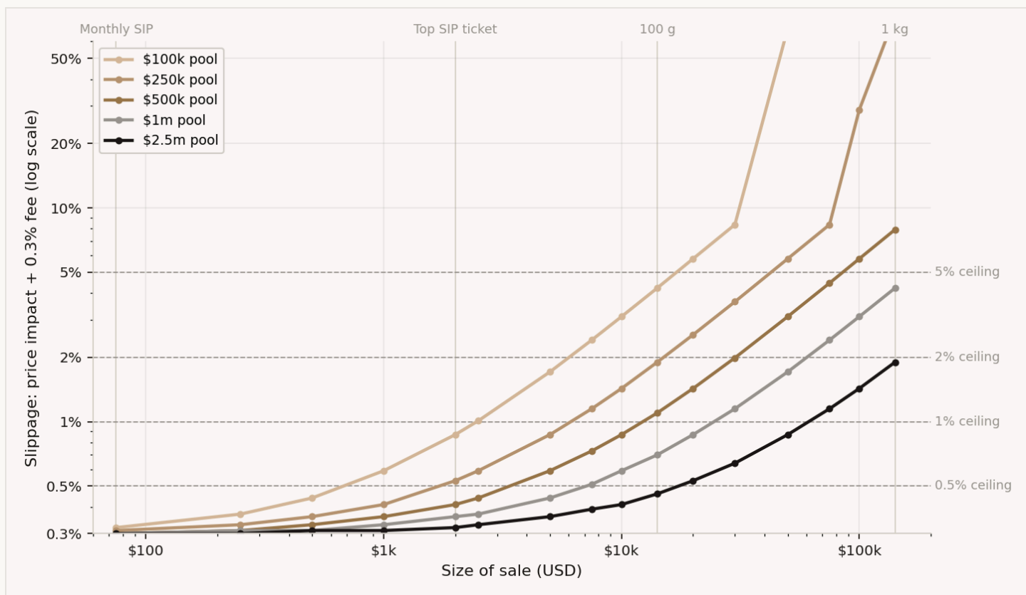
Figure 5. Slippage against sale size in a V3 \pm 10\% pool, one line per pool size
