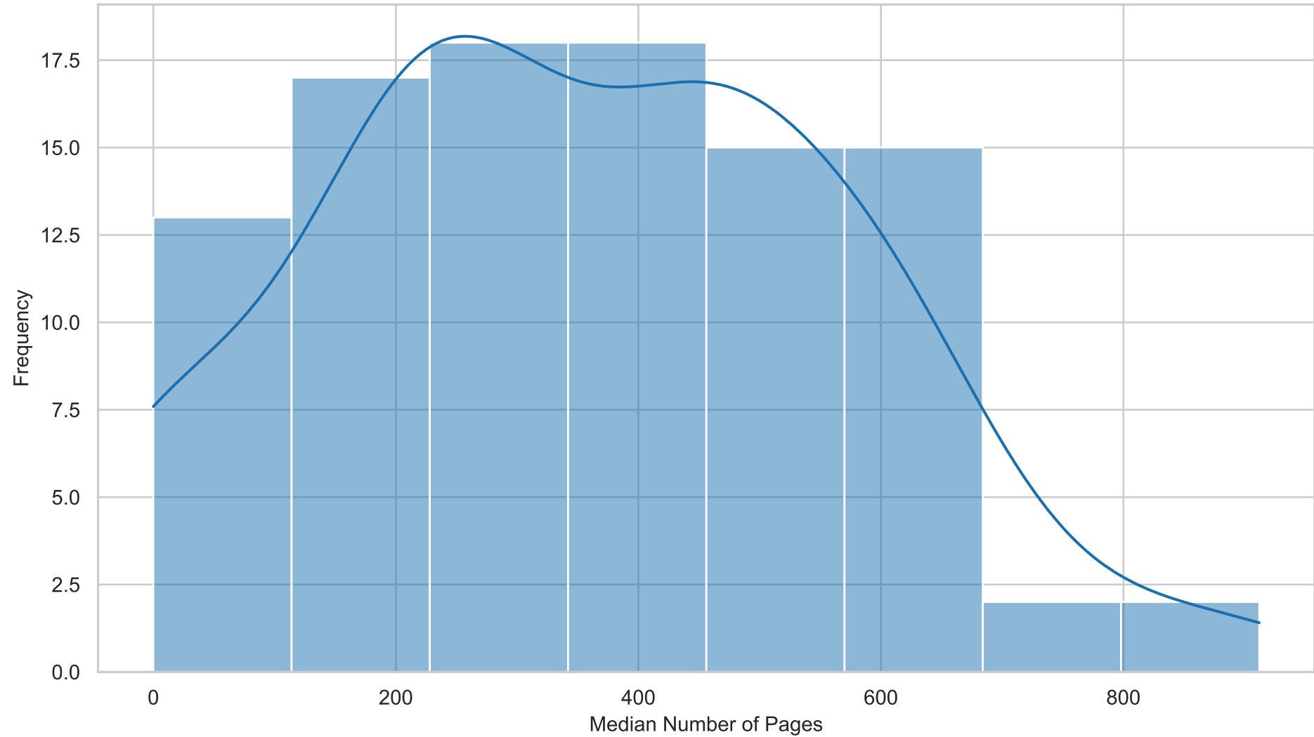
Distribution of Book Page Counts
