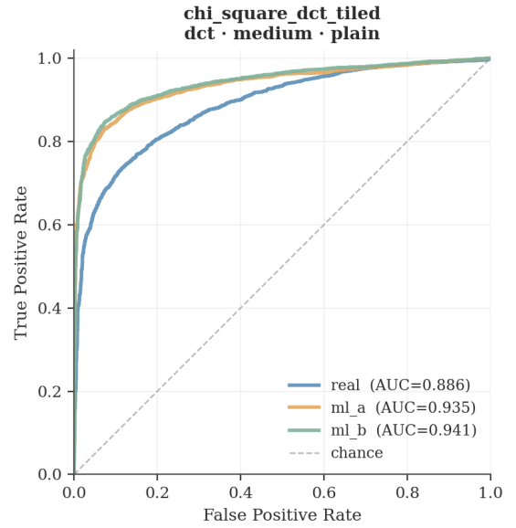
Fig. 10. ROC curves for \chi^2 -DCT-tiled at DCT/medium/plain ( N=3,000 ). The per-source ordering real (AUC=0.886) < SDXL (0.935) < FLUX (0.941) is consistent with RQ1. The global \chi^2 -DCT detector on the same data reaches only AUC=0.778, well below the tiled variant.
