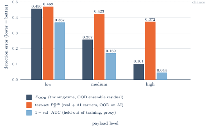
Fig. 13. DCTR under real-only training: training-time E_{\text{OOB}} (dark), in-distribution validation proxy 1 - \text{val\_AUC} (light), and operational test-set P_E^{\text{min}} on a real+AI corpus (orange). The gap between dark and orange is the cover-source-mismatch effect at the operational metric.
