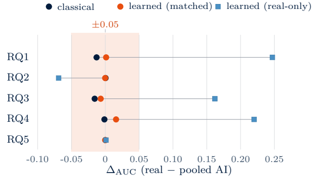
Fig. 10. Cross-validation verdicts per RQ across three detector configurations: classical (dark circle), matched-training learned (orange circle), real-only-training learned (light square). The orange band marks the pre-registered \pm 0.05 practical-significance gate. Real-only training pushes RQ1, RQ2, and RQ4 well outside the band, the central real-only finding, while classical and matched-training agree inside it. RQ3’s real-only marker is the high-payload representative (+0.162 pooled over the per-payload values \{+0.053, +0.220, +0.213\} ).
