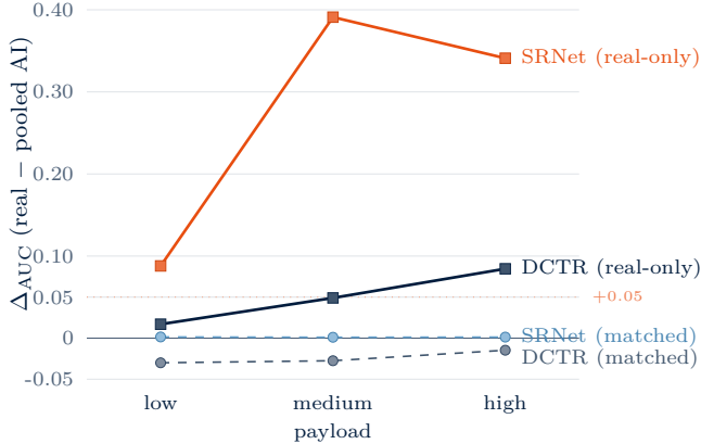
Fig. 12. Learned-detector payload trend, parallel to Fig. 7. Matched-training detectors (dashed, light markers) sit near zero, SRNet at ceiling, DCTR slightly real-harder. Real-only training (solid, square markers) flips direction and inflates the gap by 5–300×: SRNet peaks at medium payload (real-easier by +0.39 AUC), DCTR grows monotonically with payload.
