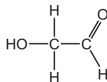
hydroxyethanal
