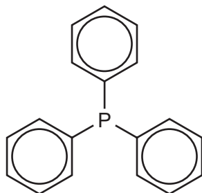
triphenylphosphine
