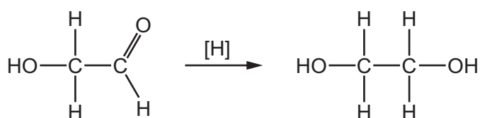
hydroxyethanal
