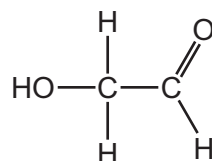
hydroxyethanal
