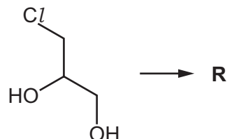
3-chloropropane-1,2-diol
