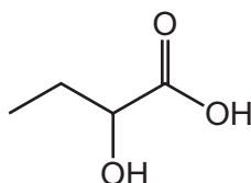
2-hydroxybutanoic acid
