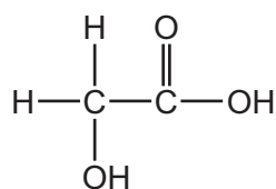
glycolic acid
