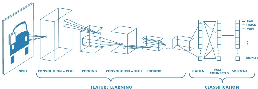
Figure 1: A simple CNN topology optimized for image classification.
