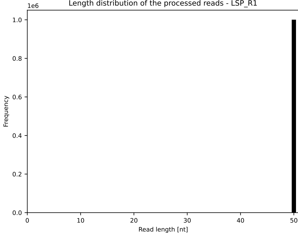
Length distribution of the processed reads - LSP_R1
