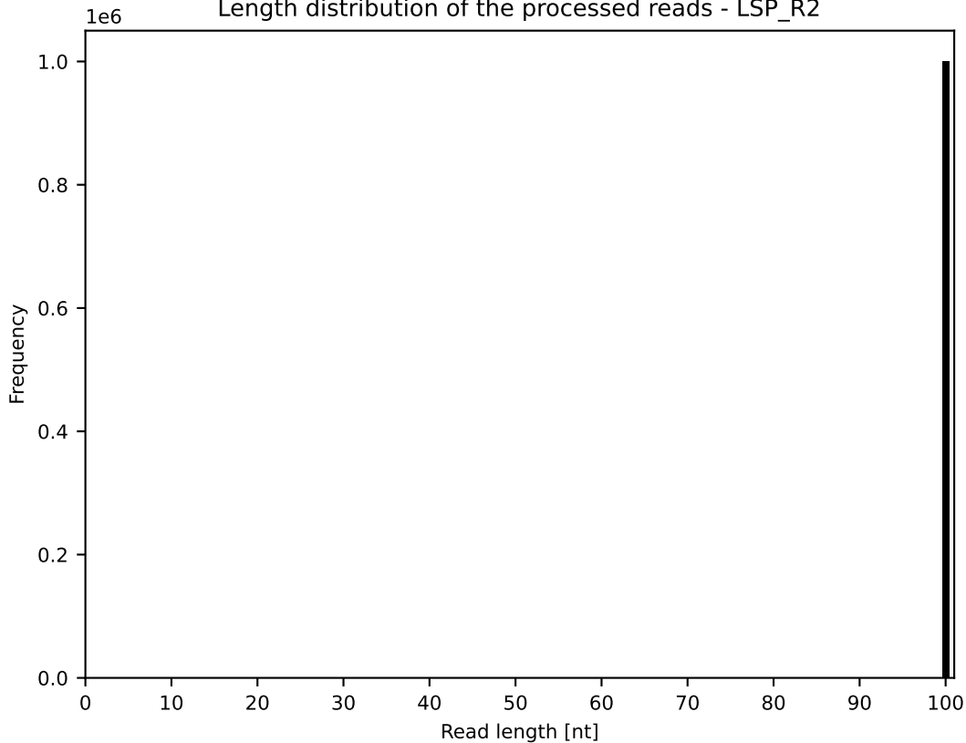
Length distribution of the processed reads - LSP_R2
