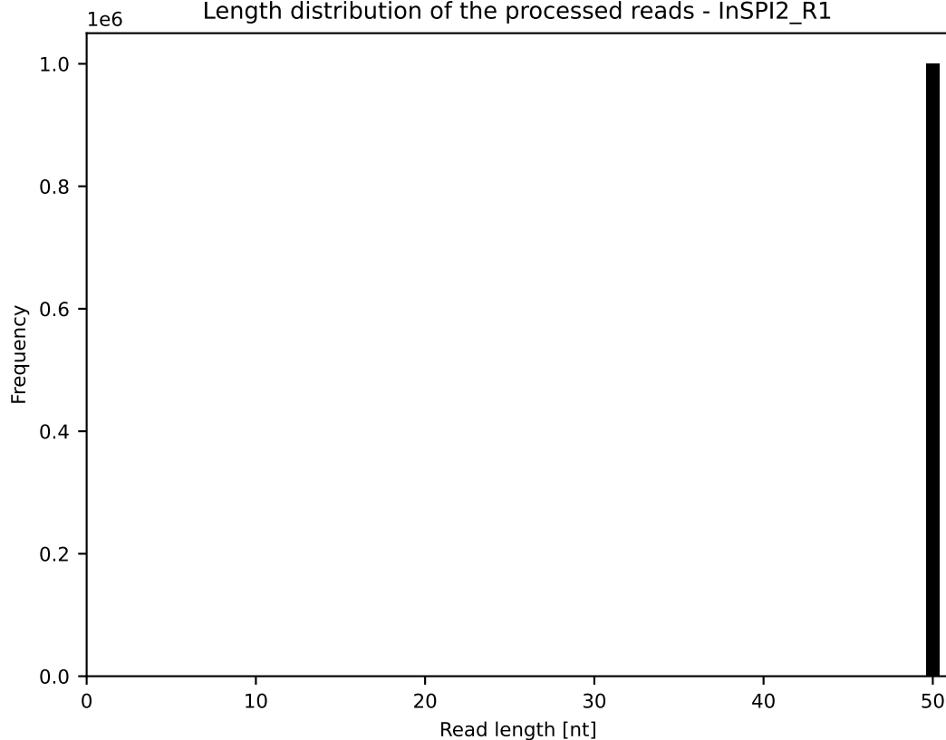
Length distribution of the processed reads - InSPI2_R1
