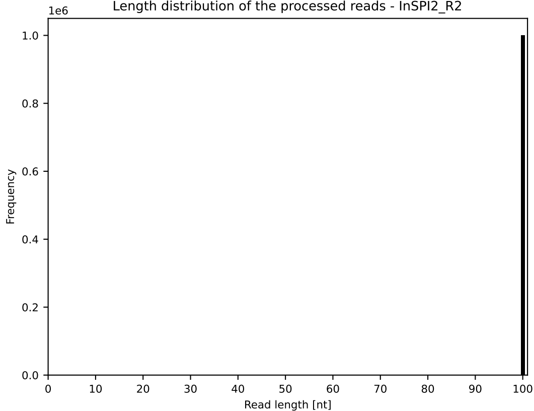
Length distribution of the processed reads - InSPI2_R2
