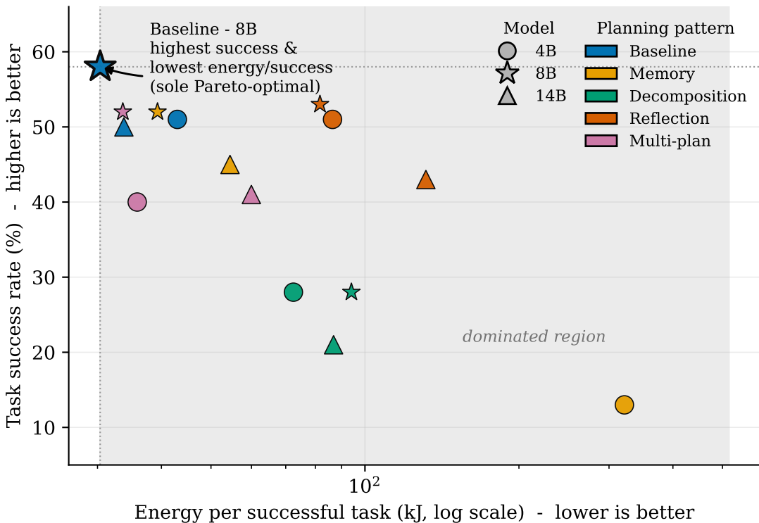
Energy-performance trade-off across all 15 configurations
