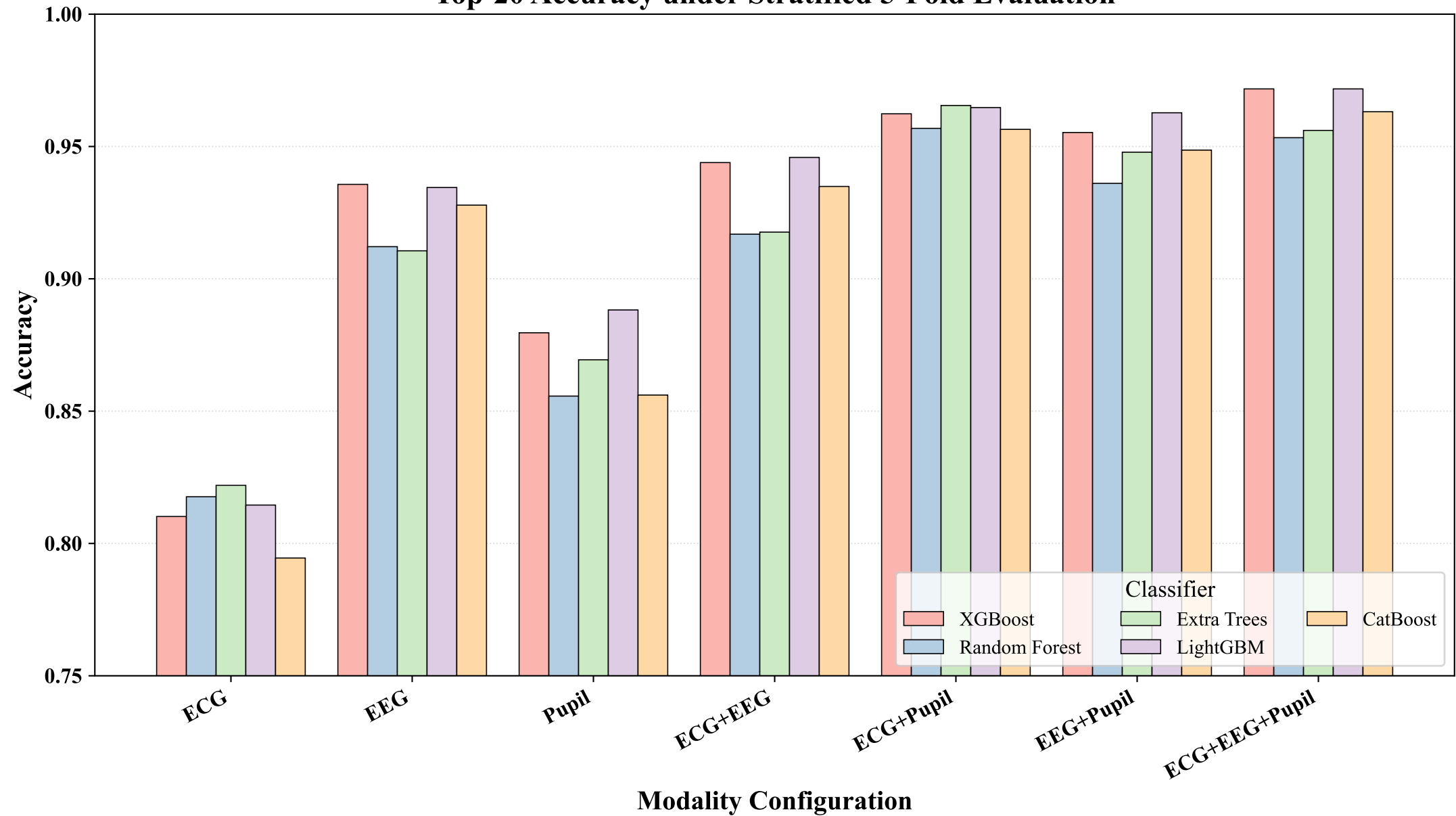
Top-20 Accuracy under Stratified 5-Fold Evaluation
