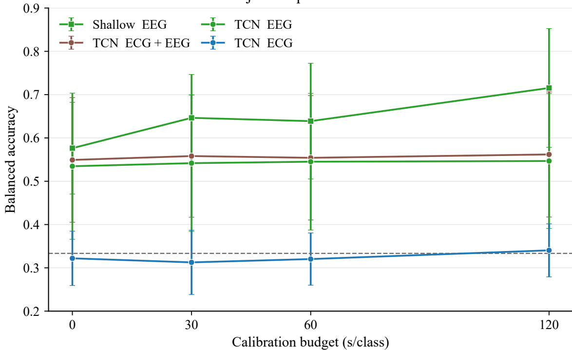
Subject-adaptive calibration
