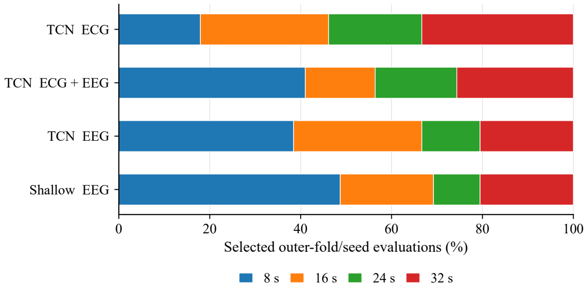
Validation-selected input duration
