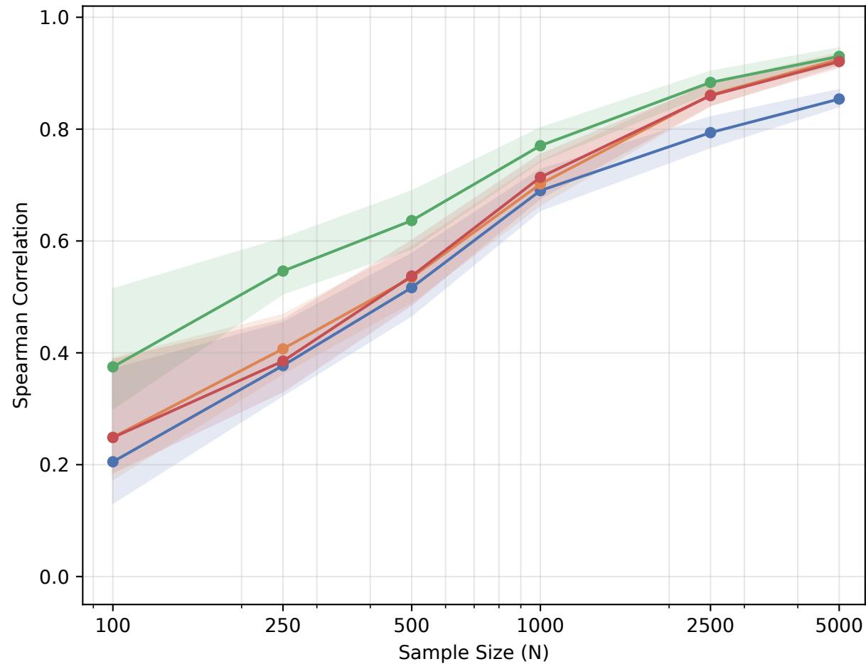
Full-Ranking Spearman Stability
