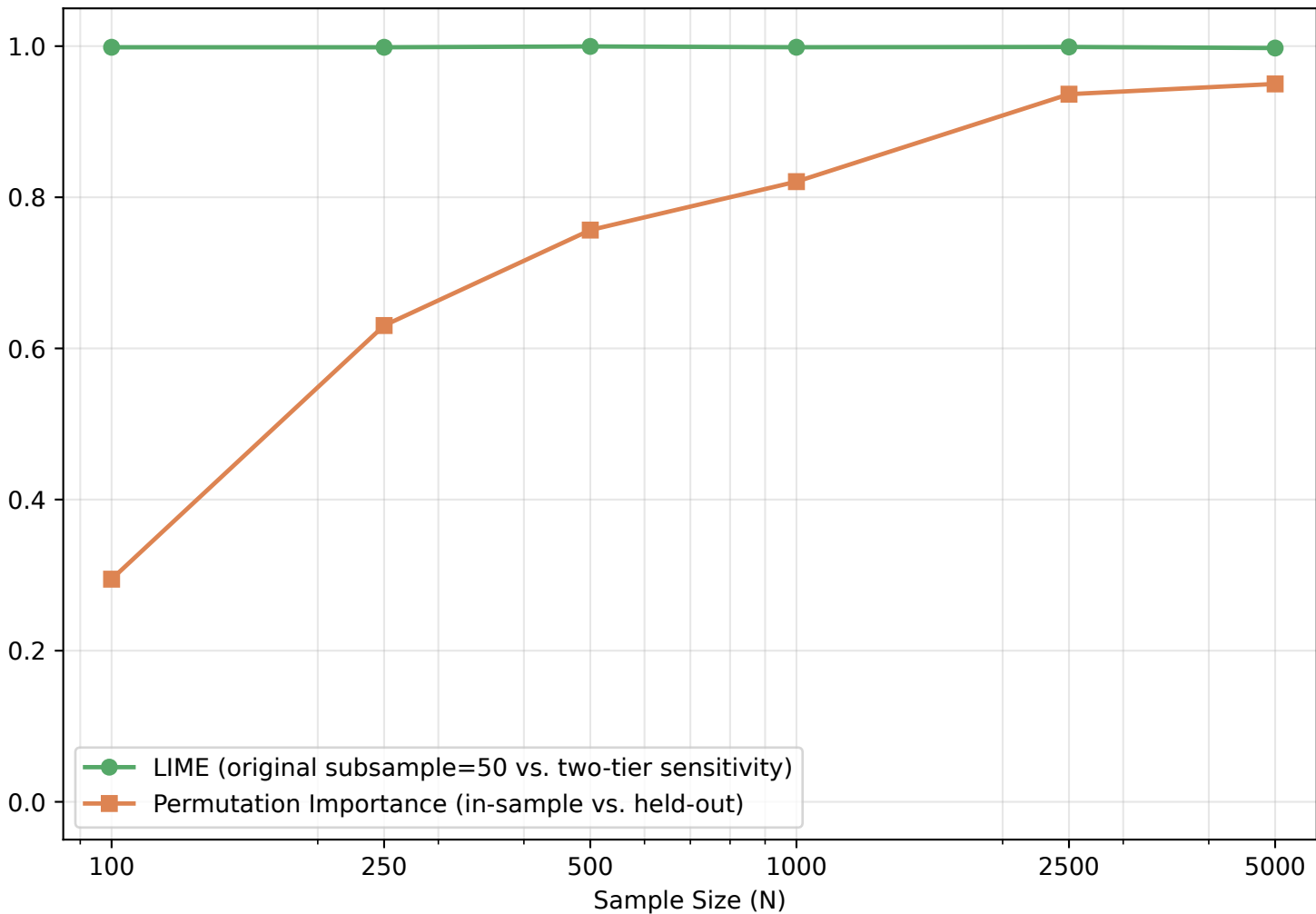
Mean Spearman Agreement with Original Ranking
