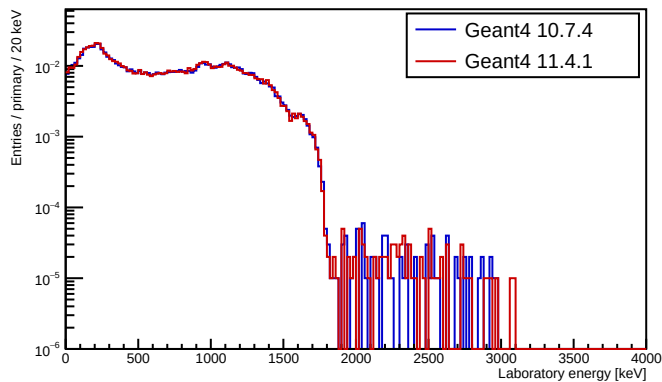
Ex = 2457 keV: crystal deposits
