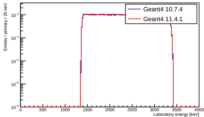
Ex = 2150 keV: recorded emitted gammas
