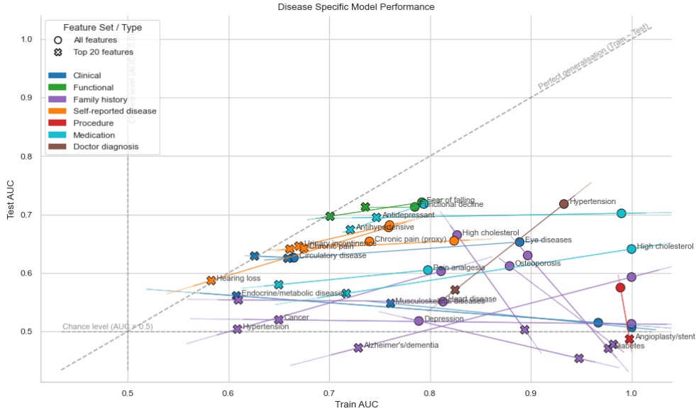
Figure 5.3: Train vs Test AUC for all Track B disease specific models, coloured by outcome category. For each disease, a circle marks the all features model, and a cross marks the top-20 model, connected by a line showing the shift between strategies. Dashed lines at 0.5 indicate chance level discrimination. Confidence ellipses show the spread of points within each outcome category.
