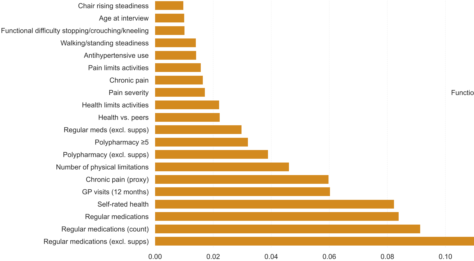
RF
