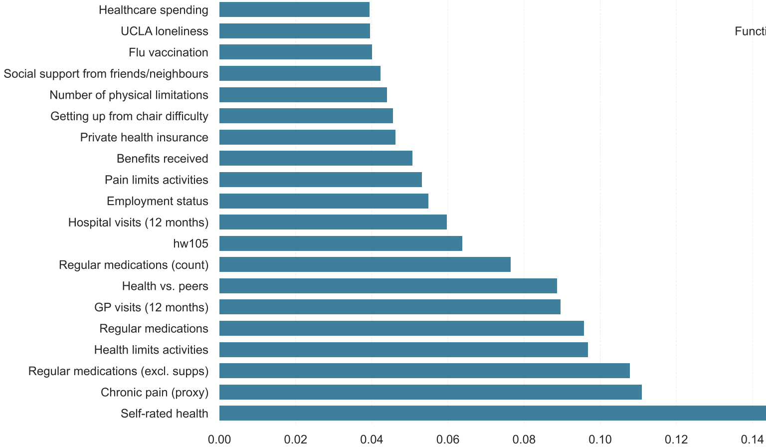
LR
