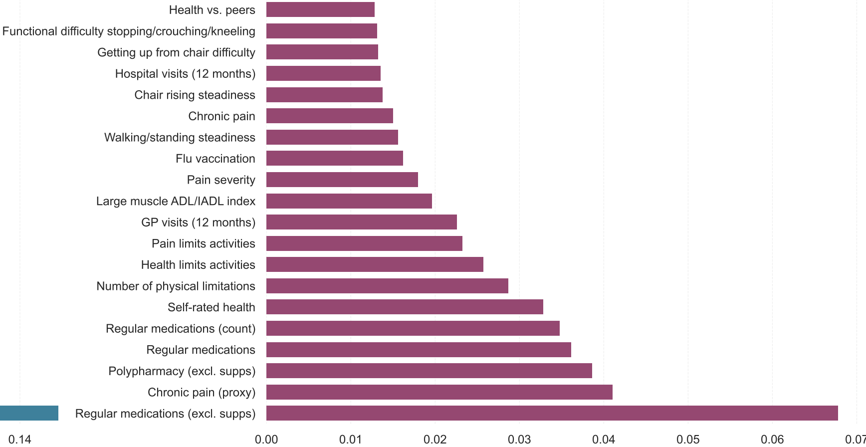
XGB
