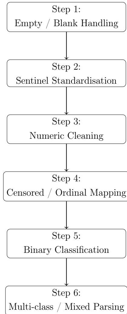
Figure 4.1: Flowchart of the final six step cleaning pipeline applied to all TILDA waves. See full transformation tables in Appendix B.7 and E for the detailed progress “.ipynb” script, at each scenario cleaning step.
