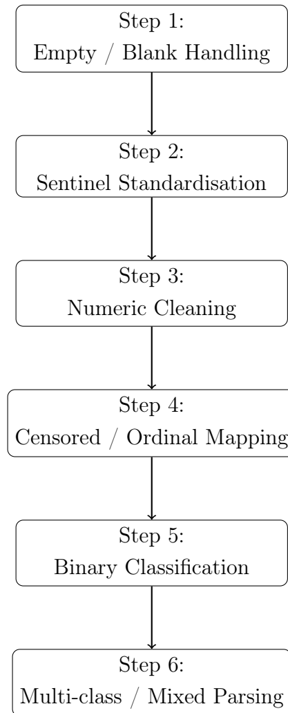
Figure 4.2: Flowchart of the final six step cleaning pipeline applied to all TILDA waves. See full transformation tables in Appendix B.7 and E for the detailed progress “.ipynb” script, at each scenario cleaning step.
